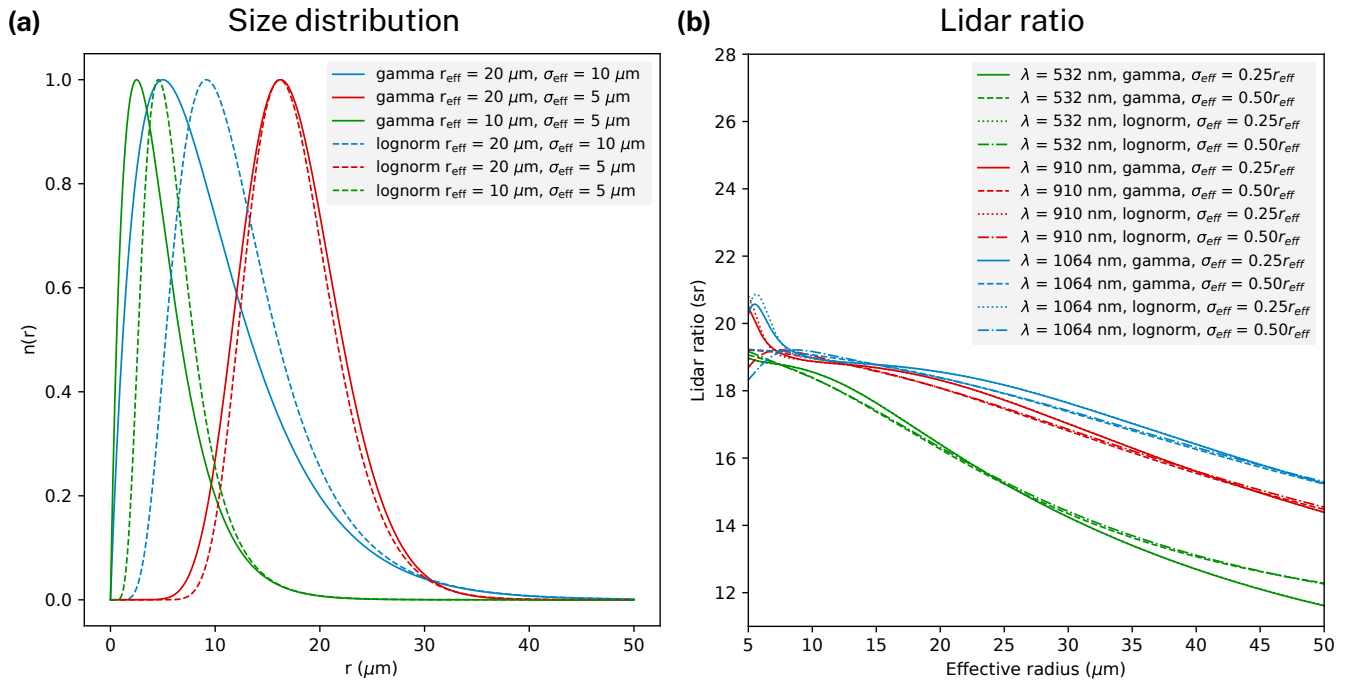
Figure 3. (a) Theoretical distributions of cloud droplet radius based on the log-normal and Gamma distributions parametrised by multiple choices of the effective radius r_{\text{eff}} and effective standard deviation \sigma_{\text{eff}} . (b) Lidar ratio (LR) as a function of effective radius calculated for different theoretical cloud droplet size distributions, laser wavelengths and effective standard deviation ratios.
