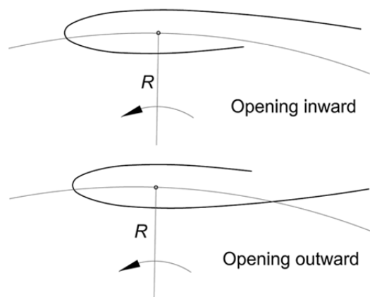
Figure 3. Opened symmetrical airfoils oriented radially inward and outward (R – rotor's radius).
