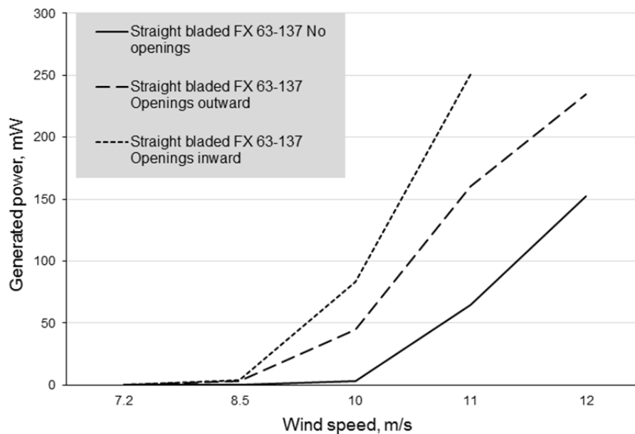
Figure 13. The turbines with full and opened blades, FX 63-137 airfoil curvature outward.
