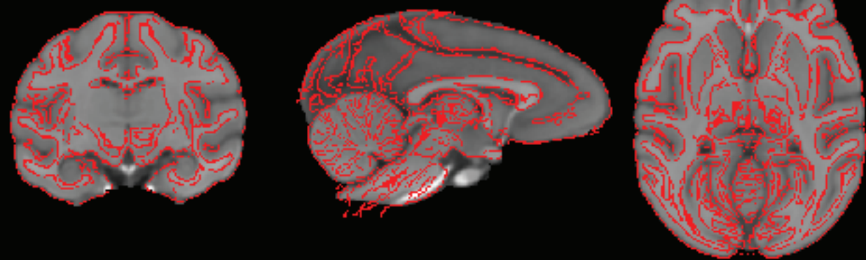
D99 edges on NMTv1.2 volume
