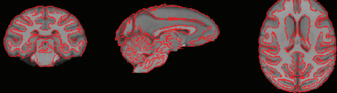
D99 edges on MNI volume
