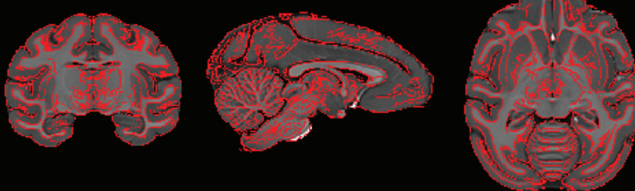
D99 edges on NMTv1.3 volume
