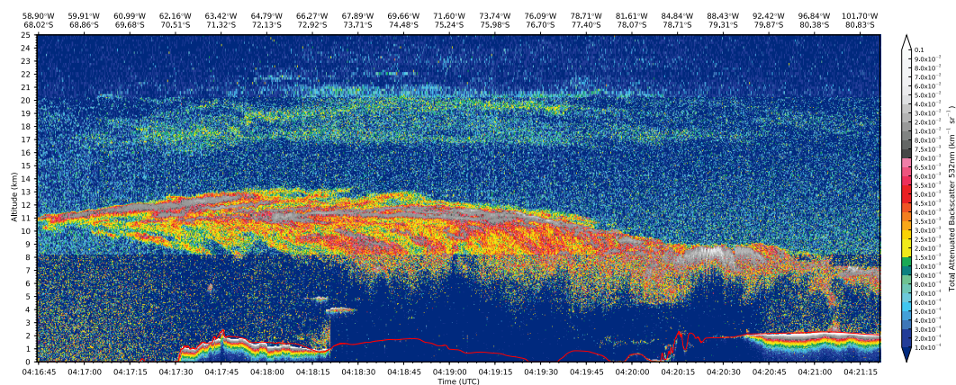
CALIPSO Profile 2007-06-12T04:16:44Z/2007-06-12T04:21:21Z
