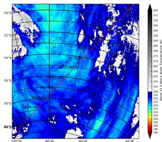
MODIS Swath, CALIPSO Trajectory 2007-06-12T04:16:47Z/2007-06-12T04:21:13Z
