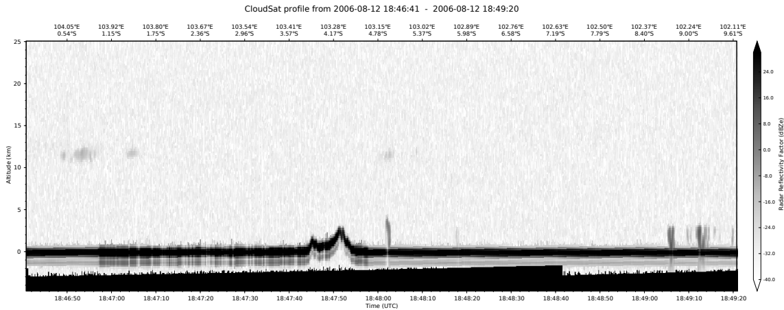
Figure 6.1 | cloudsat1.pdf
