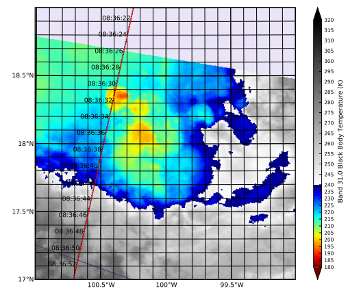
a) MODIS Swath, CALIPSO Trajectory 2007-07-16T08:36:20Z/2007-07-16T08:36:53Z
