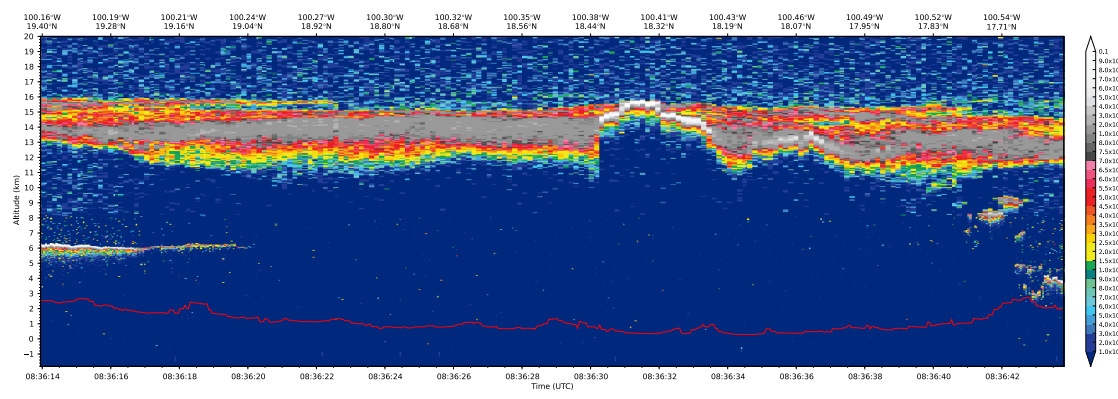
c) CALIPSO Profile 2007-07-16T08:36:14Z/2007-07-16T08:36:43Z
