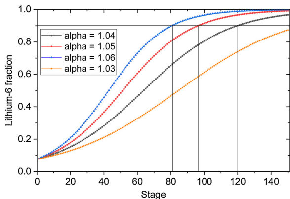
Fig. 5. Model of a separation cascade with lithium-6 fraction at S stages.
