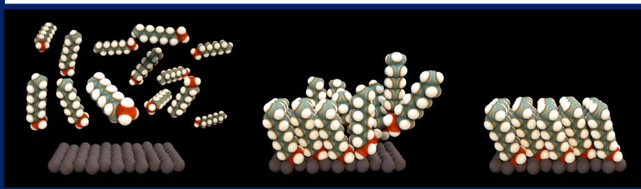
FIG. 3. Schematic illustration of the underlying adsorption and self-alignment mechanisms in a SAM process: (a) a source precursor is introduced into the reaction zone; (b) the precursor molecules are adsorbed to the substrate surface and are surface-constrained by physisorption; (c) weak forces (e.g., van der Waals, polar interaction) between the adsorbent molecules drive self-assembly and ultimate molecular orientation. The self-assembled adsorbent molecules monolayer thus become “anchored” to the substrate by relatively slow chemisorption.
