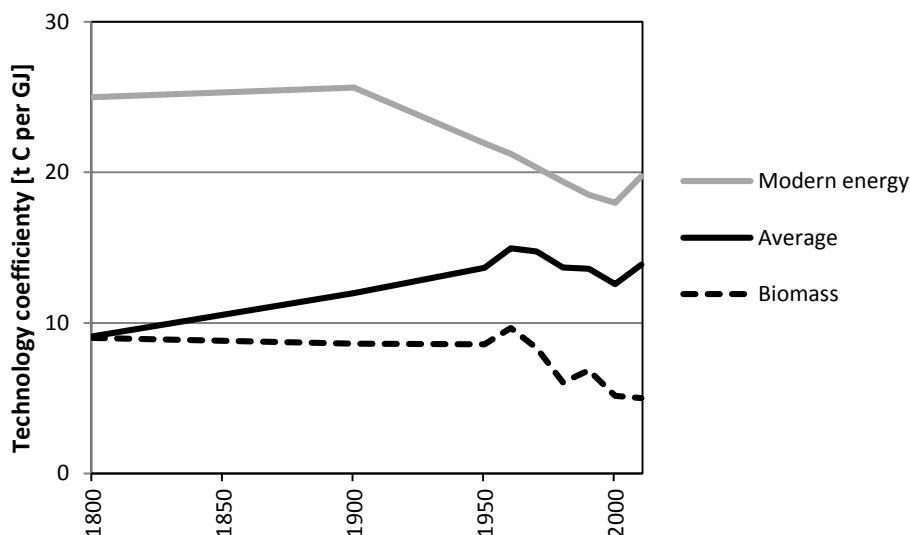
Figure 6. Development of technology coefficients for Carbon emissions in t Carbon per unit energy use (DEC).
