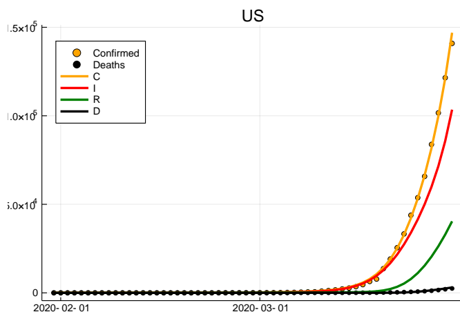
Fig. 10: Data from the US (dots) and assimilation (lines)
