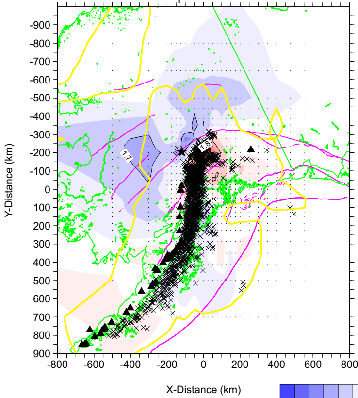
Z= 65 vpv_saku81
