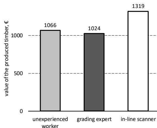
Fig. 7 The market value of assortments produced by the sawmill when implementing three diverse log sorting scenarios. The exchange rate of Euro (1 EUR = 4.30 PLN ) according to the National Bank of Poland as at 26th November 2019.
