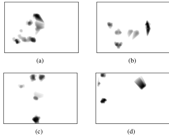
Figure 11. Examples of tactile images misclassified by HandsNet ; (a) and (b): non-human hand contacts classified as hands; (c) and (d): human hand contacts classified as non-hands.
