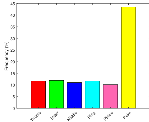
Figure 10. Histogram representing the average frequency of pixels for segmented class. The colors shown in the histogram are also used in the following to identify the segments in the tactile images.
