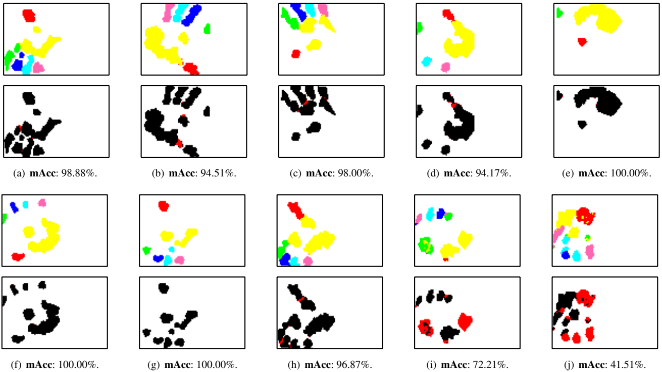
Figure 13. Examples of segmentation results. First line: SegNet output. Second line: thresholded tactile image with red areas corresponding to misclassified pixels.
