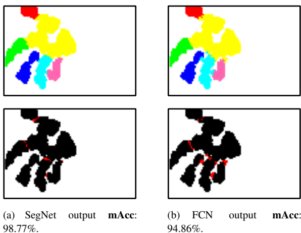
Figure 12. Segmentation performed by SegNet and FCN on the same tactile image. The first line shows the models output. The colors of the various segments are the same used in Figure 10. The second line shows the tactile image in binary scale with red pixels corresponding to misclassified regions.
