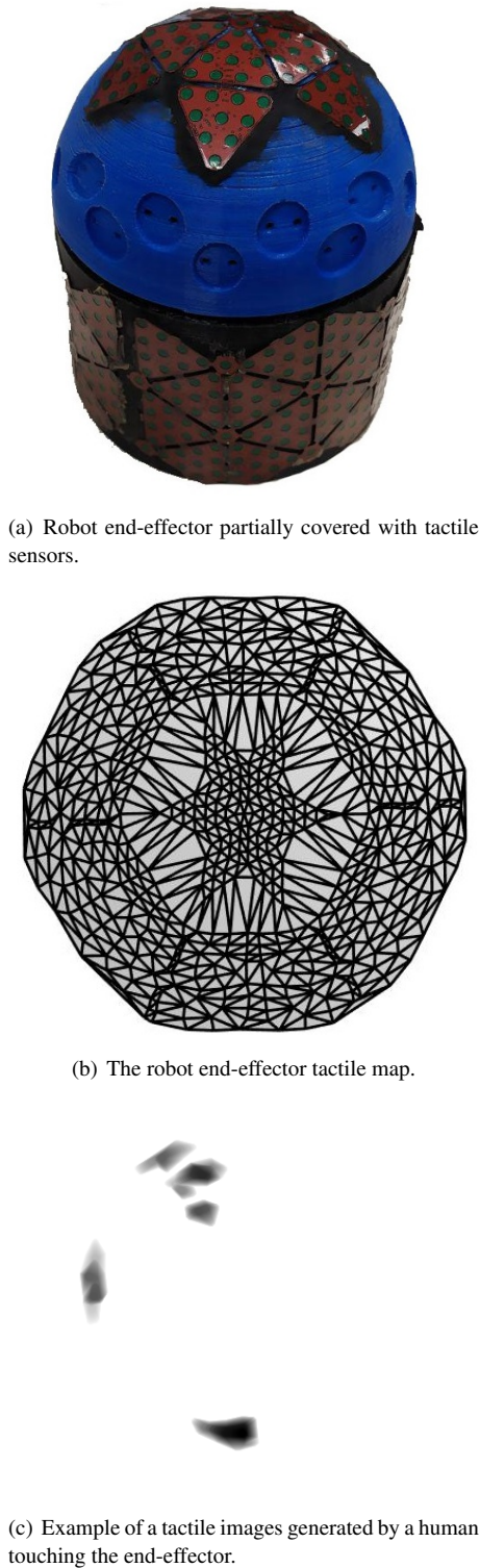
Figure 17. The sensorized robot end-effector used in this experiment.
