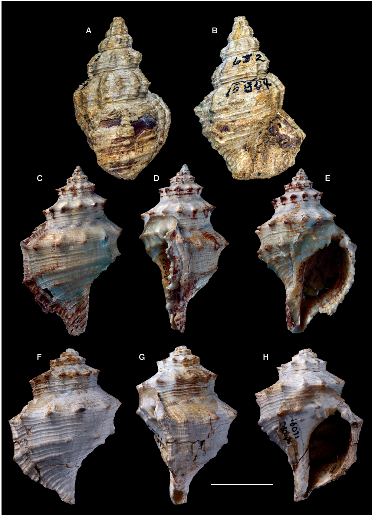
FIG. 2. — Taxa excluded from Bursidae. Olequahia Stewart, 1926 species: A, B , Olequahia domenginica (Vokes, 1939): UCMP 15804, syntype of Ranella domenginica , Tejon formation (Bartonian), California, United States; A , dorsal view; B , ventral view; C-H , Olequahia washingtoniana (Weaver, 1912): UCMP 16071 (loc. ID D8044), in dorsal ( C, F ), left lateral ( D, G ) and ventral views ( E, H ), all from Cowlitz Formation (Priabonian), Cowlitz River, Washington, United States. Scale bar: 2 cm.
