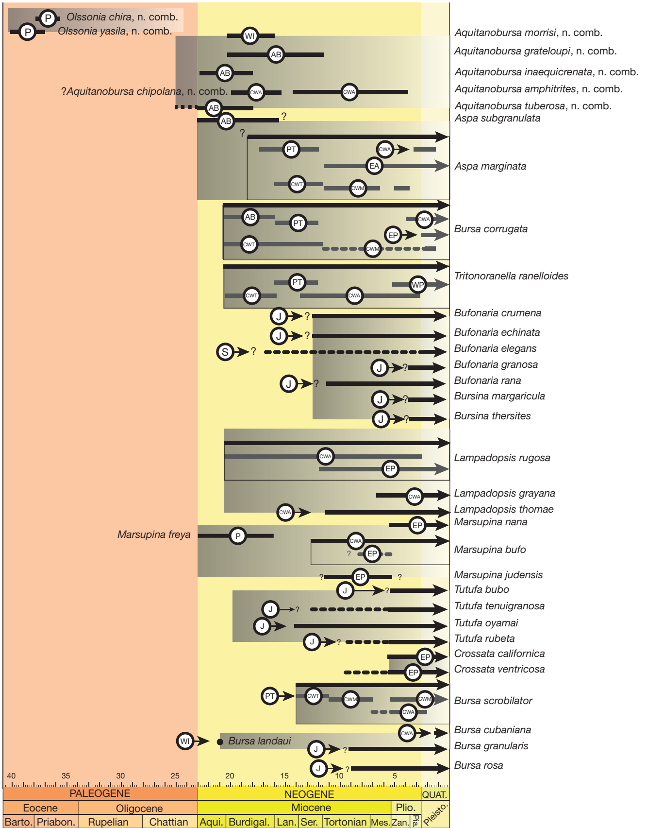
FIG. 8. — Stratigraphic range of the extinct and extant Bursidae. Black arrows indicate total stratigraphic range; grey arrows indicate regional stratigraphic range. Abbreviations: P, Peru; WI, Western Indian Ocean; AB, Aquitaine Basin; CWA, Caribbean, Western Atlantic Ocean; PT, Paratethys, CWT: Central Western Tethys; EA, Eastern Atlantic; CWM, Central Western Mediterranean; WP, Western Pacific Ocean; J, Java, Indo-Pacific; S, Sumatra, Indo-Pacific; EP, Eastern Pacific Ocean. Grey squares regroup accepted genera and putative genera within Bursa .
