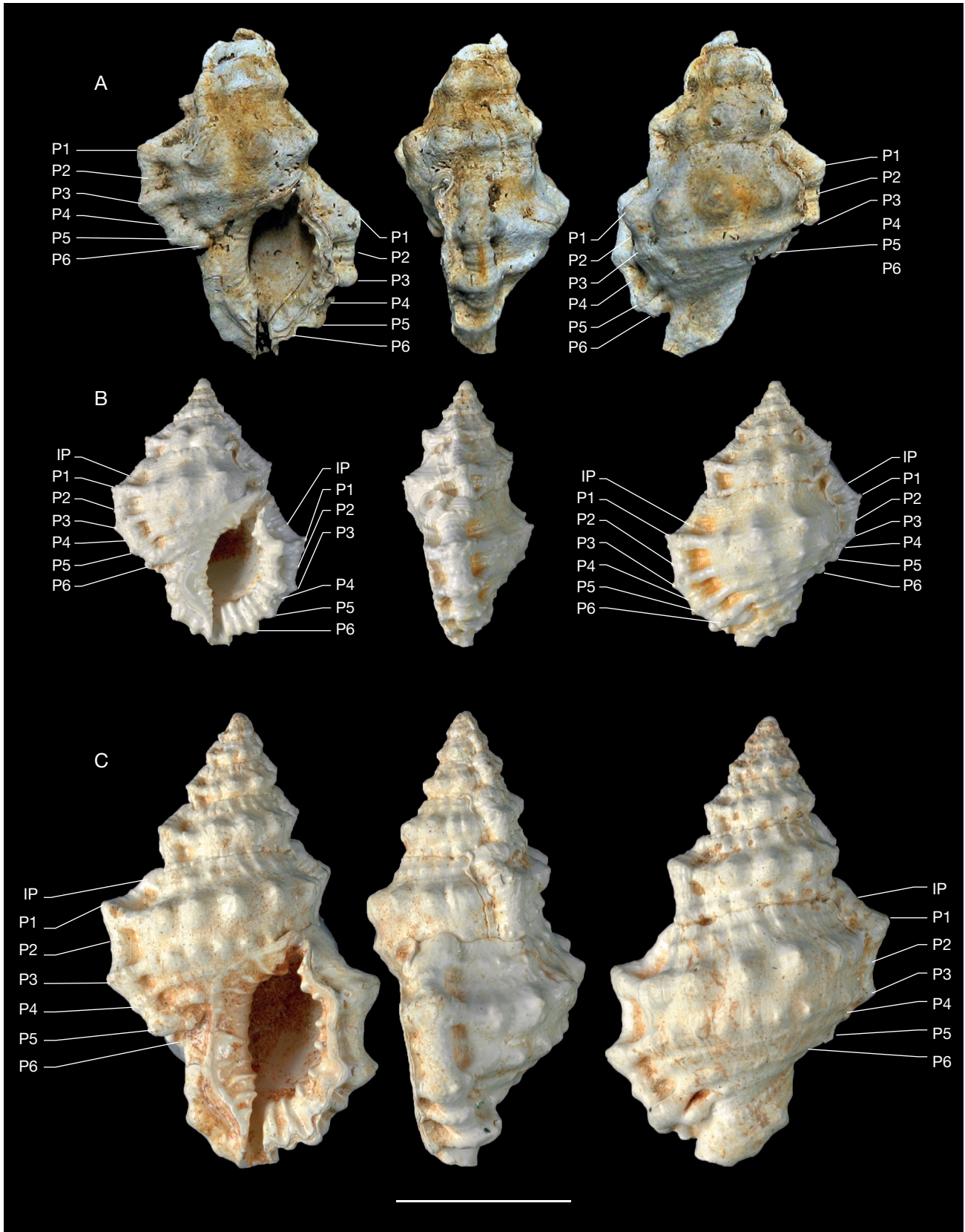
FIG. 7. — Aquitanobursa n. gen. of Aquitaine Basin: A , Aquitanobursa grateloupi (d'Orbigny, 1852) n. comb., MNHN.FA27211 , lectotype from the Aquitanian of Saint-Paul-les-Dax, France; B , Aquitanobursa inaequicrenata (Cossmann & Peyrot, 1924) n. comb., MNHN.FA70284 , Burdigalian of le Peloua, France; Faullumel coll.; C , Aquitanobursa tuberosa (Grateloup, 1833) n. comb., MNHN.FA70285 , Burdigalian of le Peloua, Staadt coll.
