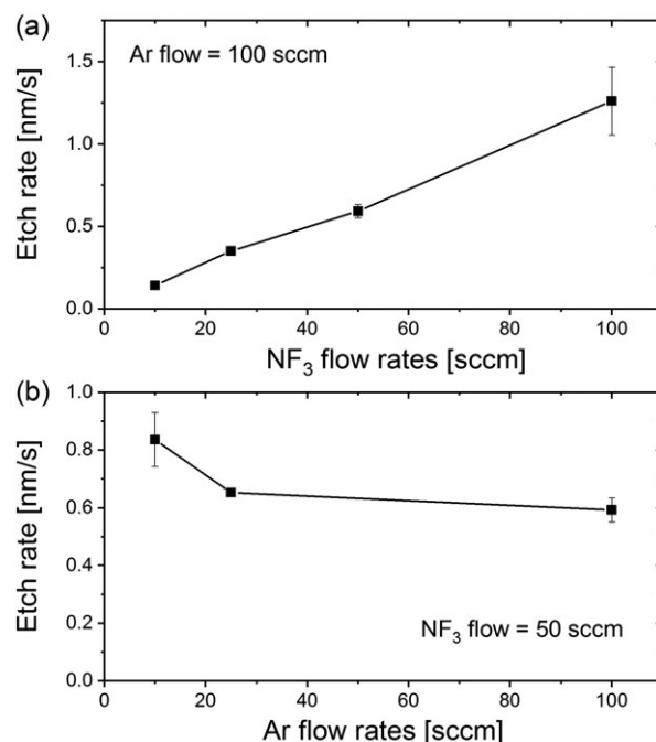
FIGURE 4 Etch rates of a-Si:H ( n^+ ) when dry etching using \text{NF}_3/\text{Ar} plasma with A, different \text{NF}_3 flow rates (at a constant Ar flow rate of 100 sccm) and B, different Ar flow rates (at a constant \text{NF}_3 flow rate of 50 sccm)
