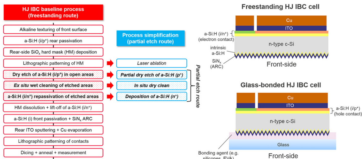
FIGURE 1 The baseline heterojunction interdigitated back contact (HJ IBC) process flow (left). Process simplifications leading to an all-dry, litho-free, cost-effective a-Si:H patterning sequence are also indicated (middle). Cross-sectional schematics of a freestanding and a glass-bonded HJ IBC cell are given on the right [Colour figure can be viewed at wileyonlinelibrary.com ]
