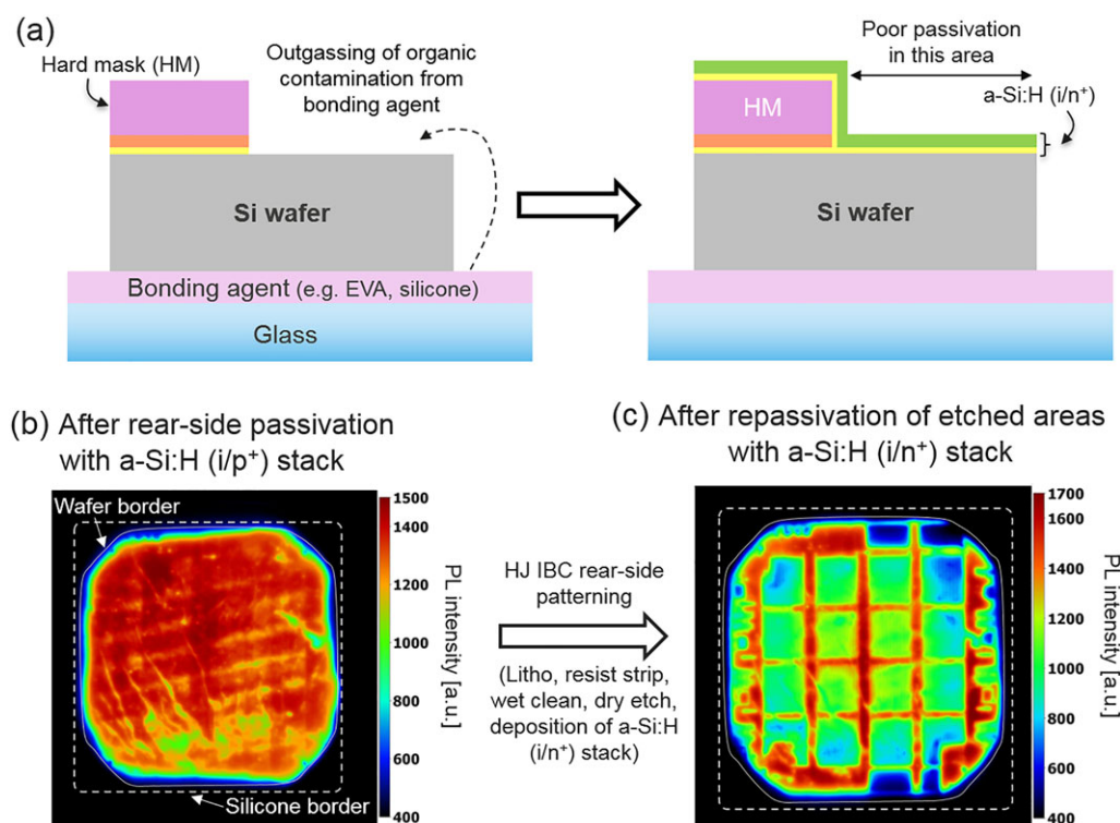
FIGURE 3 A, schematics depicting outgassing of organic contamination from the bonding agent onto the re-exposed c-Si surfaces and the resulting poor repassivation. B, and C, photoluminescence (PL) images showing the passivation quality during rear-side processing of heterojunction interdigitated back contact (HJ IBC) cells on glass-bonded silicon [Colour figure can be viewed at wileyonlinelibrary.com ]
