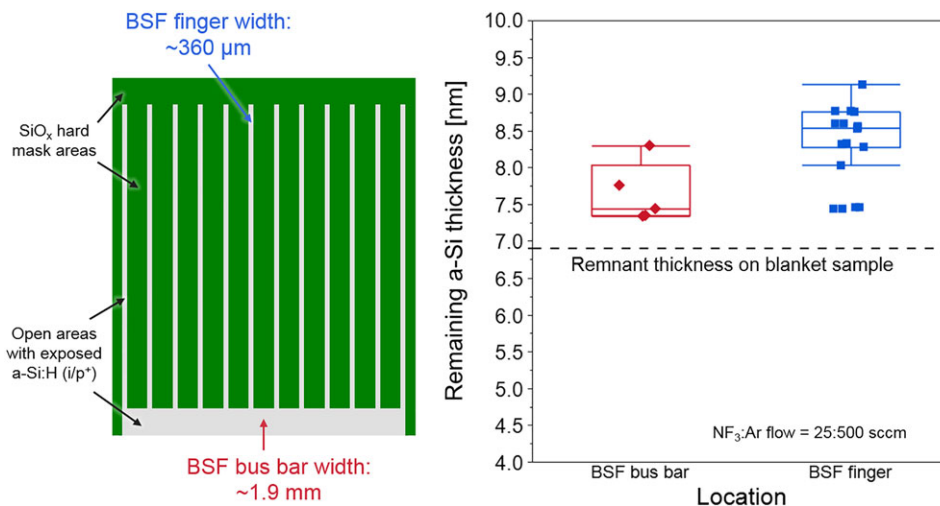
FIGURE 5 Schematic on the left shows design of our small-area IBC rear-side a-Si finger pattern. Plot on right shows the remaining a-Si:H thickness after the partial etch process at the BSF finger and bus bar areas. The dashed line indicates the expected thickness on blanket samples [Colour figure can be viewed at wileyonlinelibrary.com ]
