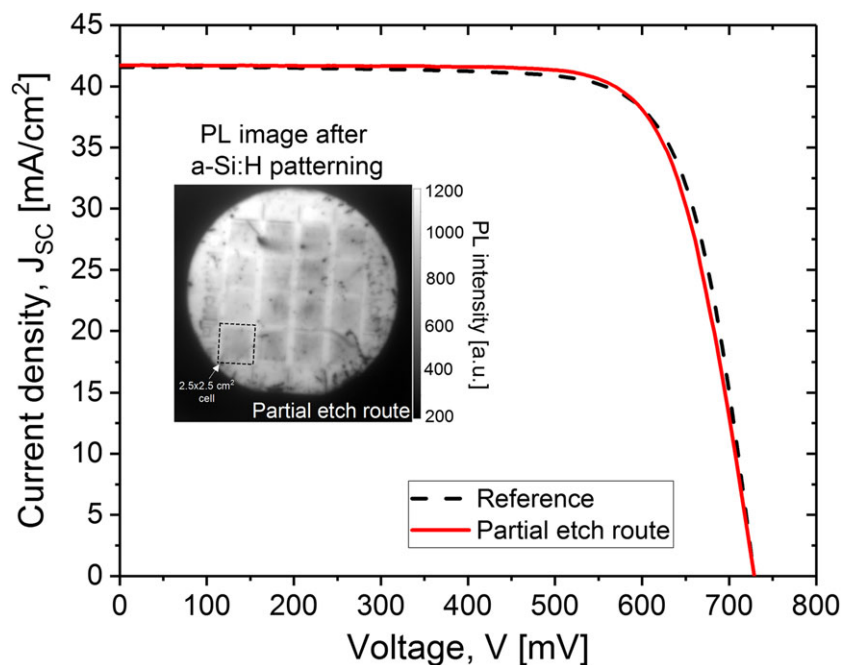
FIGURE 9 The current–voltage characteristics under AM1.5G illumination of the best cell from the partial etch route and that from the reference conventional process sequence. Inset shows the uncalibrated PL image of a wafer after the rear-side a-Si:H patterning, from the partial etch route [Colour figure can be viewed at wileyonlinelibrary.com ]
