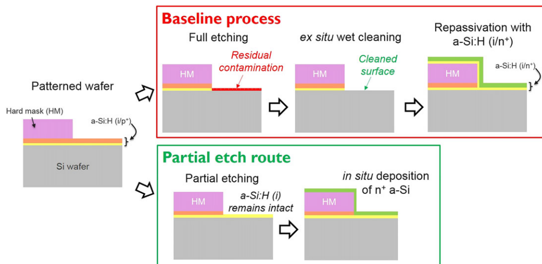
FIGURE 2 Schematics depicting the steps after hard mask (HM) patterning till the realization of interdigitated strips of a-Si:H (i/p + ) and a-Si:H (i/n + ), comparing the conventional baseline route with the proposed partial etch route [Colour figure can be viewed at wileyonlinelibrary.com ]
