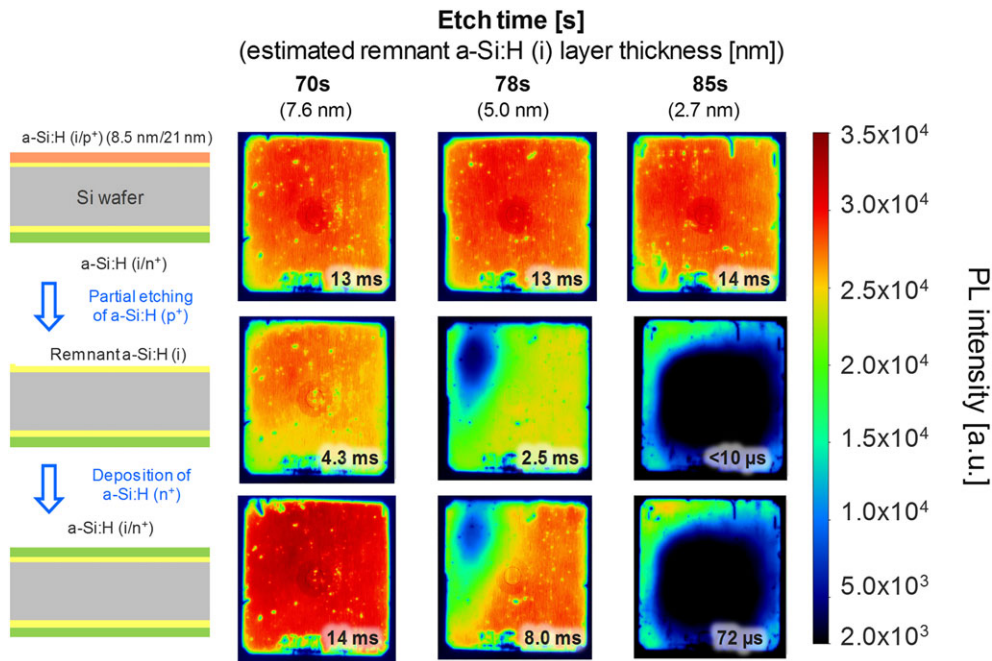
FIGURE 6 Schematics on the left depict the three stages of the process sequence: A, after passivation, B, after partial etch of the p-doped a-Si:H layer on the front, and C, after deposition of the n-doped a-Si:H layer. The PL images corresponding to these stages are given on the right, where the partial etch time is varied from 70 seconds to 85 seconds, resulting in the estimated remnant a-Si:H thickness ranging from 7.6 nm to 2.7 nm. The minority carrier lifetime at an injection level of 10^{15} \text{ cm}^{-3} is given inside the PL images, for all cases, except for the ones with lifetime below 100 \mu s, where the highest lifetime reached in low-injection is mentioned [Colour figure can be viewed at wileyonlinelibrary.com ]
