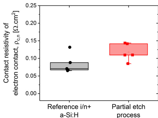
FIGURE 8 Plot of the contact resistivity values at the a-Si:H (i/n + )/ITO/Cu contact, comparing the partial etch process with reference [Colour figure can be viewed at wileyonlinelibrary.com ]
