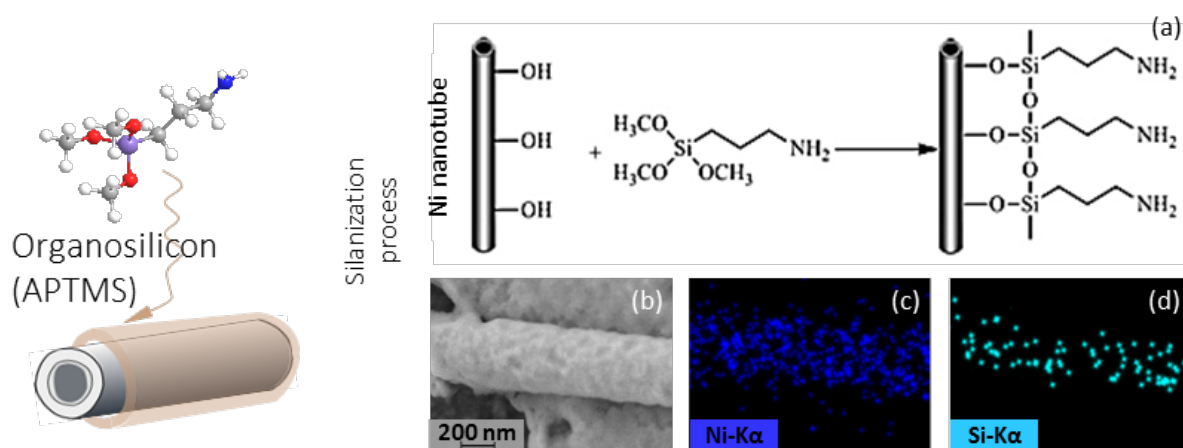
Figure 7. (a) Scheme of Ni NTs with APTMS coating. (b) SEM image of Ni NTs with APTMS coating and (c, d) EDX mapping in the regime of Ni and Si detection.
