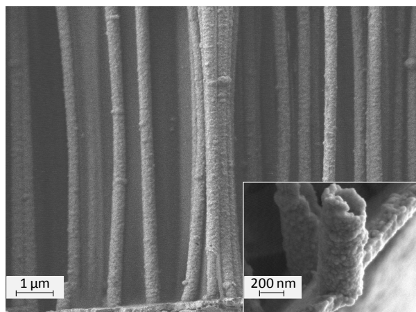
Figure 2. Typical SEM image of array of nickel nanotubes after removal from polymer template and an enlarged part of a broken nanotube (insert to the figure).
