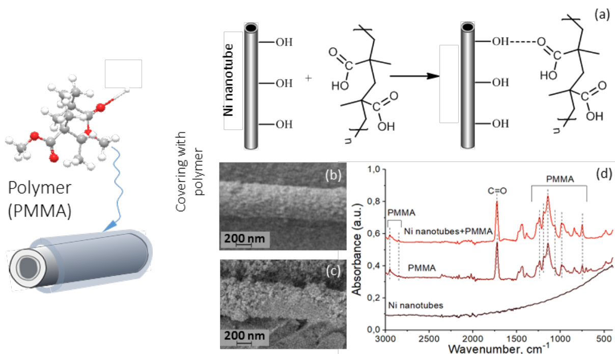
Figure 8. (a) Scheme of Ni NTs coating with PMMA. SEM image of (b) Ni NTs and (c) PMMA/Ni system. (d) FTIR spectra of coating.
