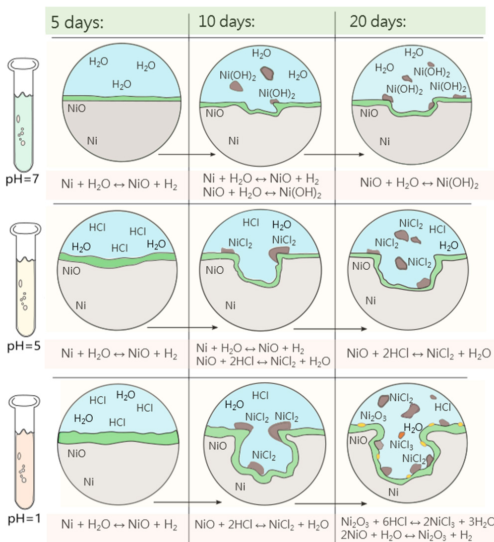
Figure 4. Schematic representation of degradation processes on the surface of Ni NTs in media with pH=1, 5 and 7 (exposition time of 5, 10 and 20 days).
