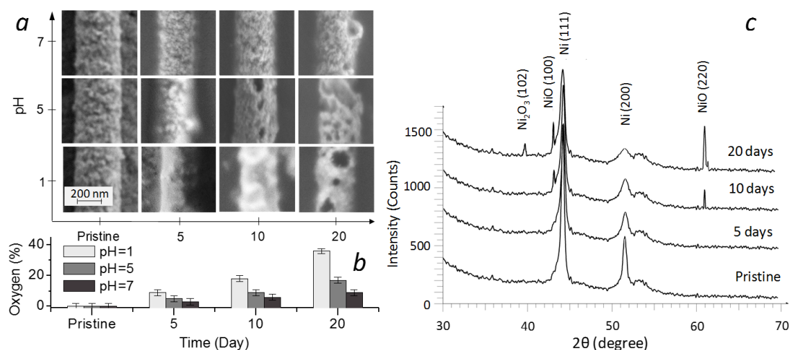
Figure 3. Degradation of Ni nanotubes depending on the time of exposition in solutions: (a) SEM images of the evolution of nickel nanotubes morphology exposition in media with different pH (scale is same for all
