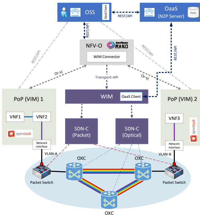
Fig. 1: Functional Architecture
