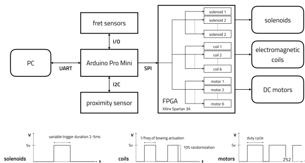
Figure 3: Hardware and command signals for the system.
