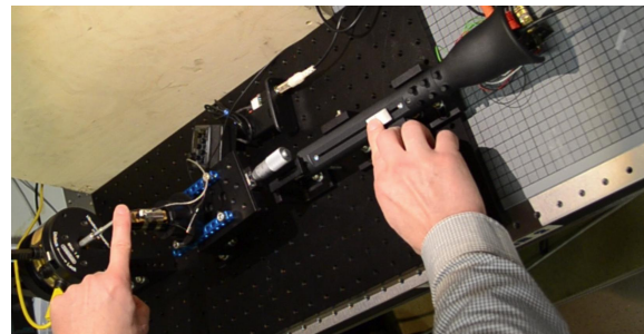
Figure 3: Setup with mouthpiece, shaker and 3D-printed controller of the half-physler.
