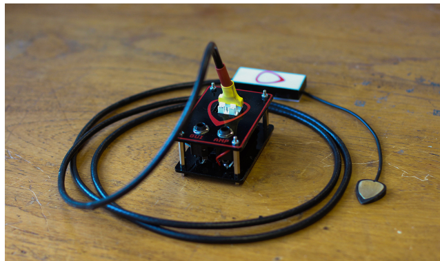
Figure 7: The Magpick system. Bela is embedded in the custom-design box in the centre.
