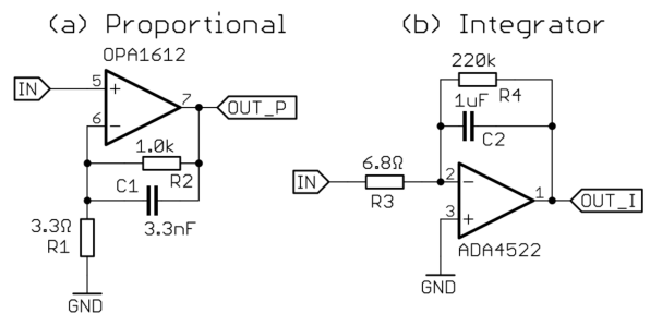
Figure 3: Schematics of the two preamplifiers.
