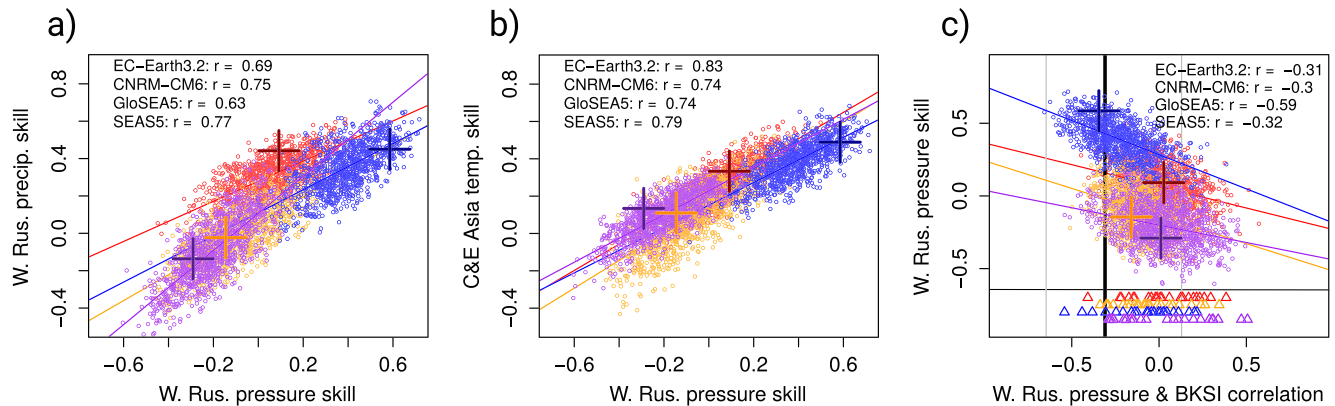
Figure 3. Scatterplots with the DJF skill relationship between (a) sea level pressure ( x axis) and precipitation ( y axis) in western Russia, (b) sea level pressure in western Russia ( x axis) and surface air temperature in northern central and East Asia ( y axis), and (c) the correlation between western Russia sea level pressure and November BKSJ index ( x axis) and the skill in western Russia SLP ( y axis). Red, yellow, blue, and purple points display values from EC-Earth3.2, CNRM-CM6-1, GloSea5, and SEAS5, respectively. All displayed r values are significantly different from 0 at the 0.05 confidence level using a one-sided T test after a Fisher transformation. The dark colored crosses represent the values from the full ensembles, while the triangles at the bottom represent the strength of the teleconnection of individual ensemble members. The black and gray vertical lines show the mean and 95% confidence interval of the correlation between ERA-Interim sea level pressure and CERSAT sea ice cover, respectively.
