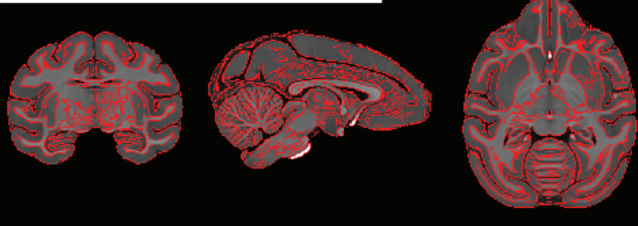
NMTv1.3 edges on YRK volume
