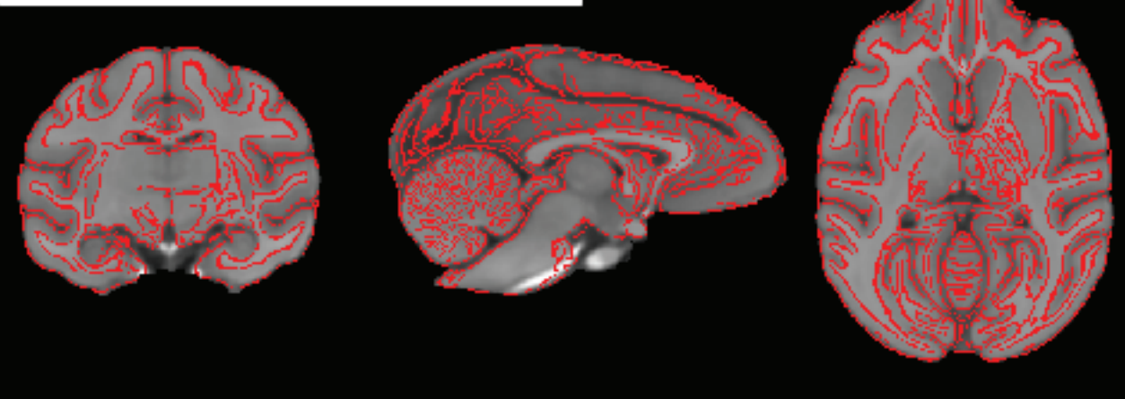
NMTv1.3 edges on NMTv1.2 volume
