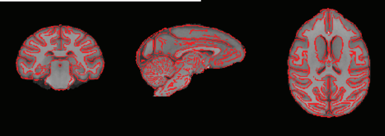
NMTv1.3 edges on MNI volume
