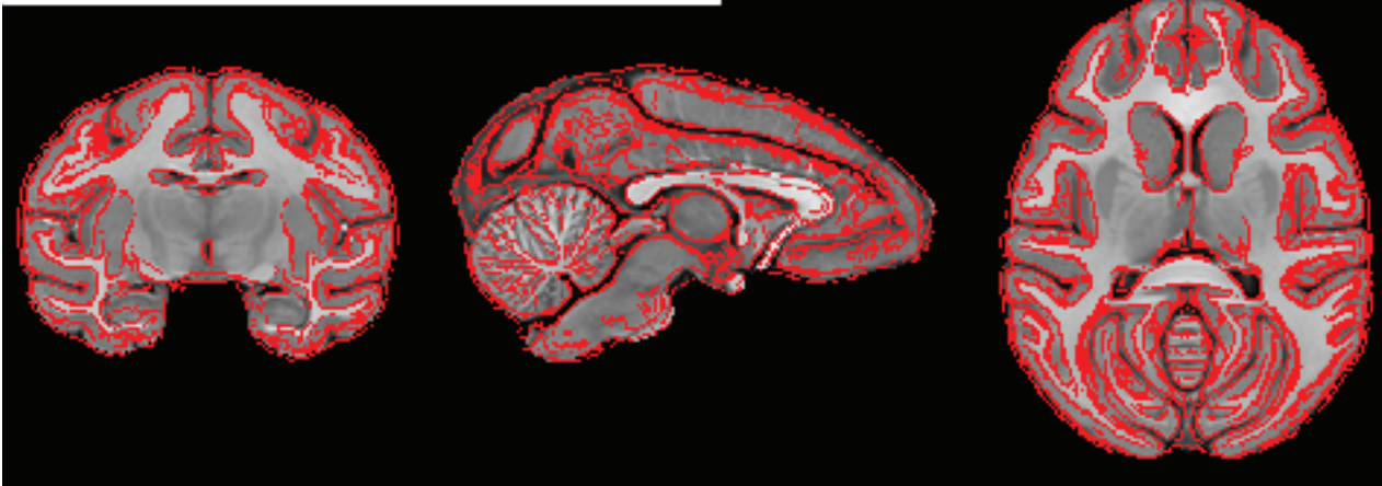
MNI edges on NMTv1.3 volume
