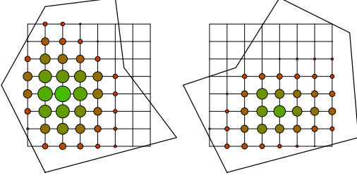
Figure 3: Uniform grid with quality metric evaluation for each candidate. A large green point represents good, a small red one bad quality
