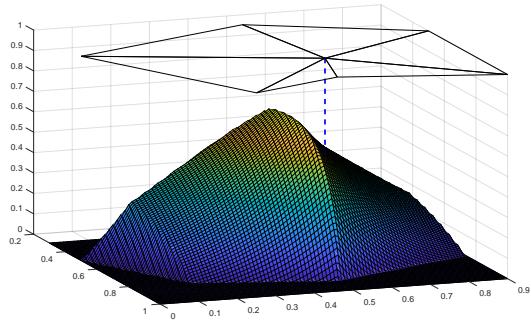
Figure 1: Vertex quality q^{(v)} according to Equation (1) with q^{(e)} defined as the mean ratio metric.
