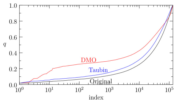
Figure 14: Comparison of Taubin smoothing and DMO on surface mesh shoe .
