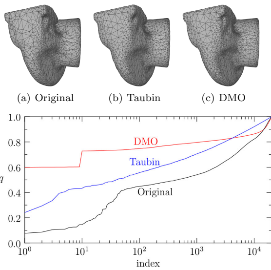
Figure 11: Comparison of Taubin smoothing and DMO on surface mesh rocker-arm .
