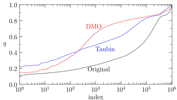
Figure 13: Comparison of Taubin smoothing and DMO on surface mesh filigree .
