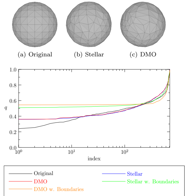
Figure 18: Volume mesh sphere .
