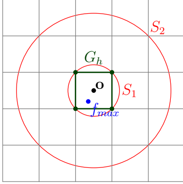
Figure 9: The best candidate of grid cell G_h must have a larger value than any point on S_2 to guarantee convergence towards f_{\max} .
