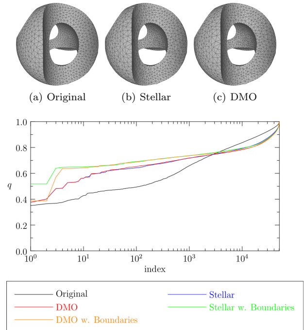
Figure 19: Volume mesh sculpt .
