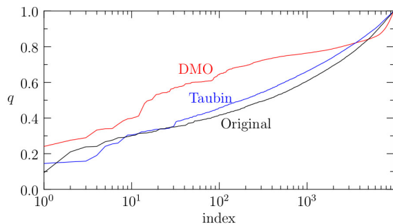
Figure 15: Comparison of Taubin smoothing and DMO on surface mesh augustus .
