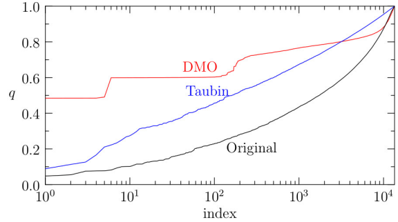
Figure 10: Comparison of Taubin smoothing and DMO on surface mesh tweety .
