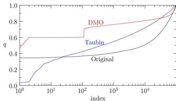
Figure 12: Comparison of Taubin smoothing and DMO on surface mesh hand .
