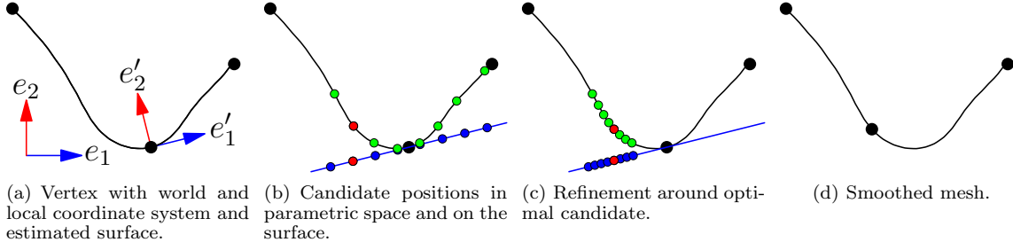
Figure 8: DMO on surface mesh. The blue line represents the parameter space on which the vertices are distributed uniformly.
