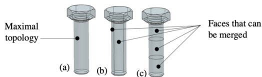
Figure 14 Examples of different boundary decomposition for the same shape. (a) The maximal topology (all faces and edges having
