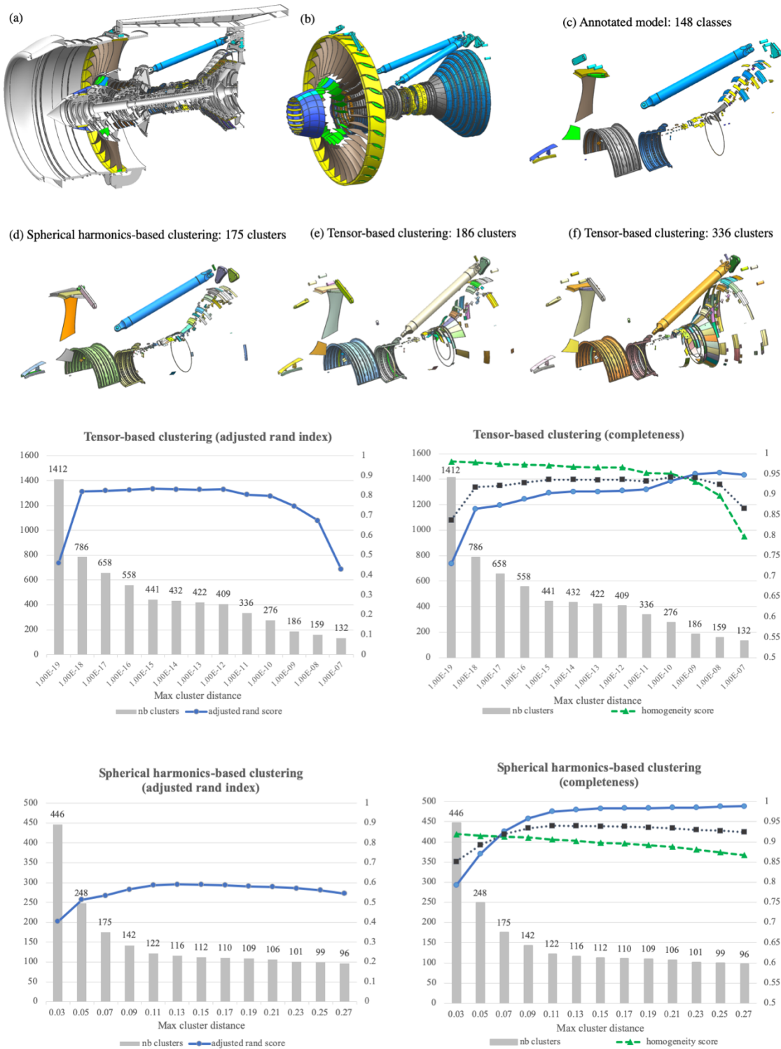
Figure 13 Evaluation of the clustering task on the Vesta model (courtesy of Rolls-Royce Plc) using the adjusted rand score and completeness score metrics: (a) the initial annotated model containing 6218 annotated solids (in color) of 6503; (b) display of the annotated solid; (c) Ground truth model containing 148 classes (one displayed component corresponds to one class), (d) clustering result based on spherical harmonics descriptors [10], (e-f) clustering result using our approach.
