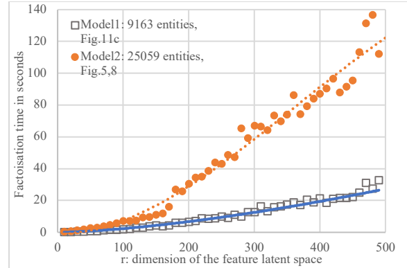
Figure 11 Evolution of the dimension of the feature latent space on the computation time to factorise the tensor.
