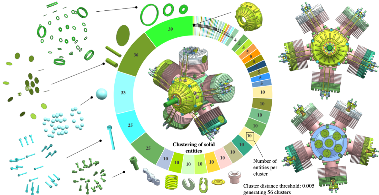
Figure 8 Application of a hierarchical clustering algorithm. The A matrix is used as input for the clustering algorithm. For this model, with a distance threshold of 0.005, 56 clusters of solid entities are generated
