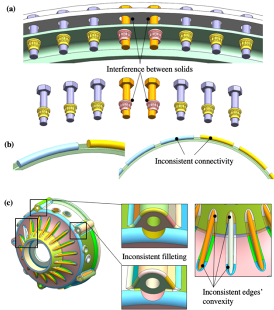
Figure 9 Example of modelling inconsistencies found following the link-based clustering task.
