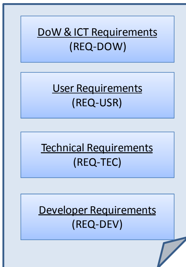
Figure 8: Requirements Categories
