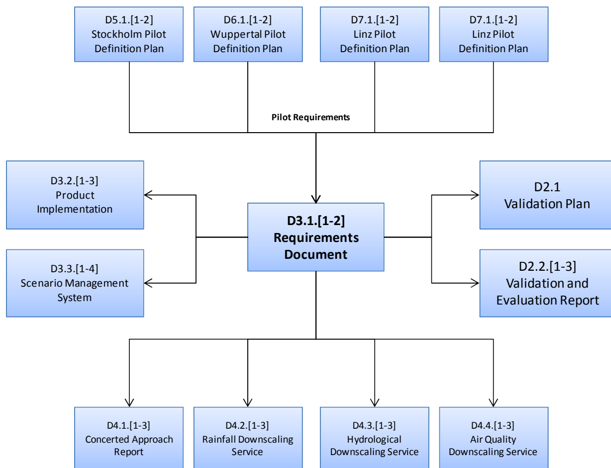
Figure 5: Documents involved
