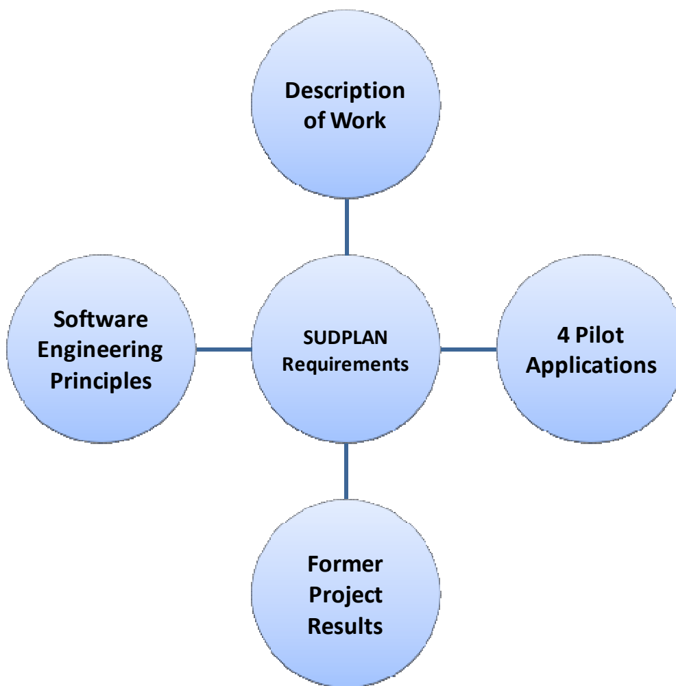
Figure 9: Requirement Sources
