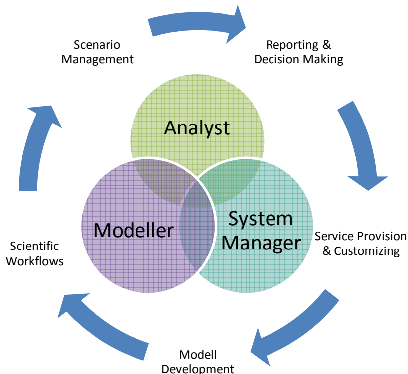
Figure 10: User Categories
