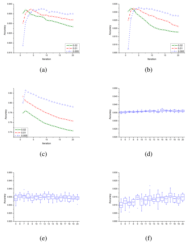
Fig. 2 Comparison of performance based on iterations (a. LiC , 10% class noise; b. LiC , 20% class noise; c. LiC , 30% class noise; d. AdaBC , 10% class noise; e. AdaBC , 20% class noise; f. AdaBC , 30% class noise)
