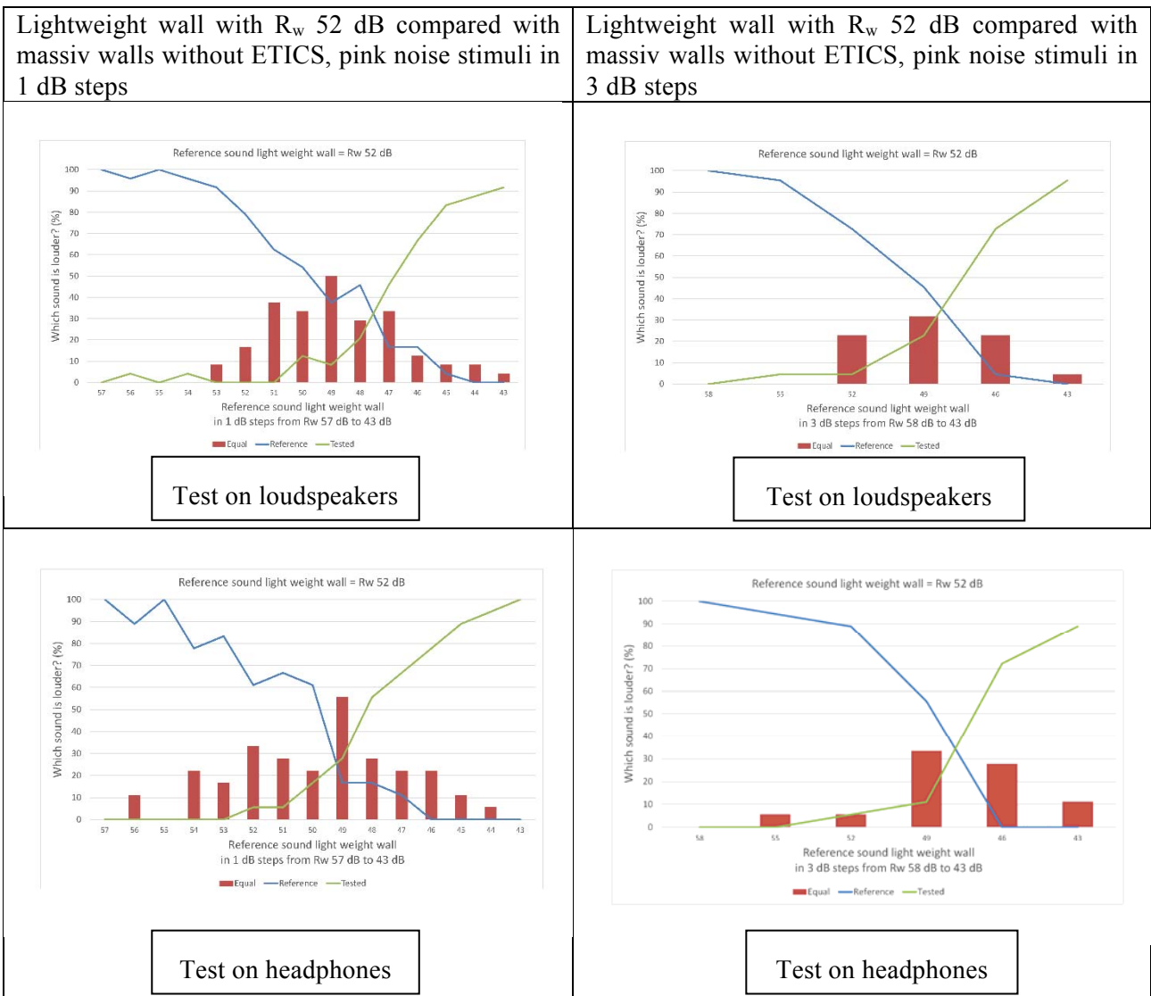
Figure 5. Shows the results of pink noise stimuli through a lightweight walls compared with massiv walls without ETICS.
