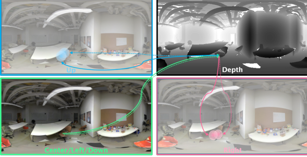
Figure 4. Depth-image-based view synthesis. For each pixel, its reprojection to another viewpoint (in horizontal or vertical stereo placement) is calculated via the estimated depth map. For each pixel a weighted splat is added to an empty canvas around its immediate reprojection neighborhood. Subsequent to their accumulation, a normalization step produces the final rendering. In this way, occlusions and irregular pixels mappings are handled gracefully, allowing for the use of view synthesis as a supervision objective, even for severe distortion areas.
