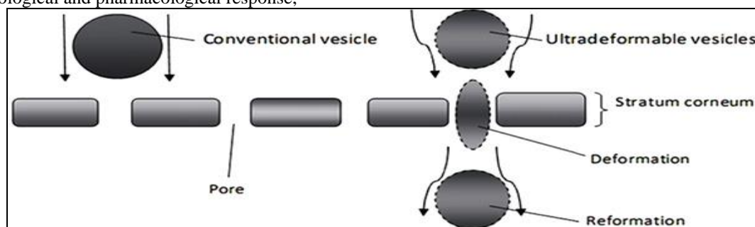
Figure 2: Schematic diagram of the two microroutes of penetration.
