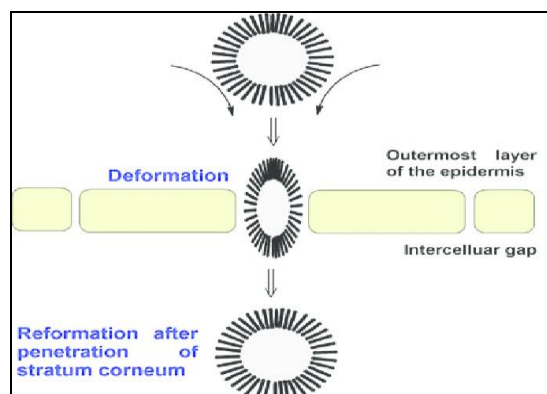
Figure 4: Penetration pathway of transfersomes
