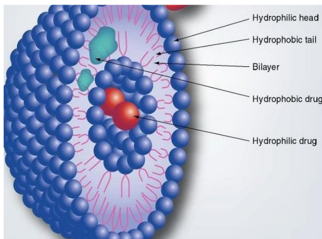
Figure 1: Structure of Transfersome
