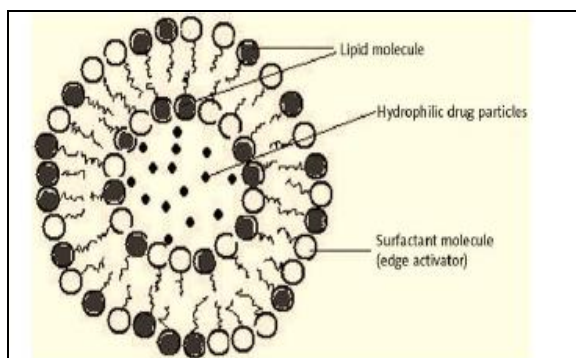
Figure 3: Structural representation of one transfersome unit Salient features of Transfersomes
