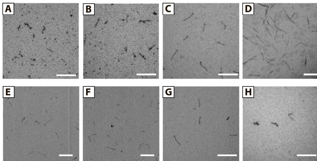
Fig. 5 TEM images of F3E10 /Dox complexes with molar ratio 50 : 1 (A), 20 : 1 (B), 10 : 1 (C), 5 : 1 (D). Images of 10 : 1 complex, diluted 10 times below CAC of F3E10 after 24 h (E) and 48 h (F). F3E10 /Iri (G) and F3E10 /doxycycline (H) with molar ratio 10 : 1. Scale bar 200 nm.
