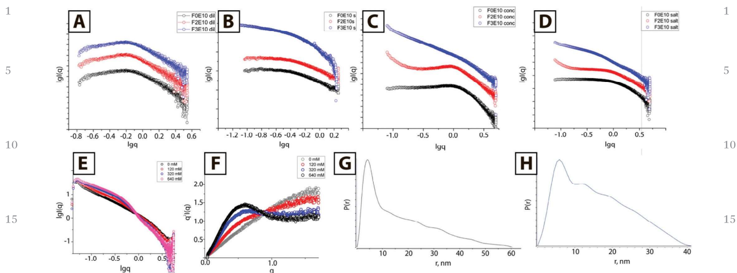
Fig. 4 SAXS profiles of FOE10 , F2E10 , and F3E10 at 0.5 mM and 3.5 mM in water (A and C) and 120 mM NaCl (B and D, respectively). SAXS curves (E) and Kratky plots (F) for F3E10 at 3.5 mM and 0–640 mM NaCl concentration. P(r) -distribution function for F3E10 (G) and F3 (H).
