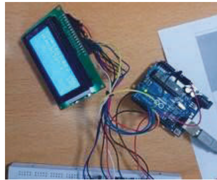
Figure 2: Arduino & LCD connections
