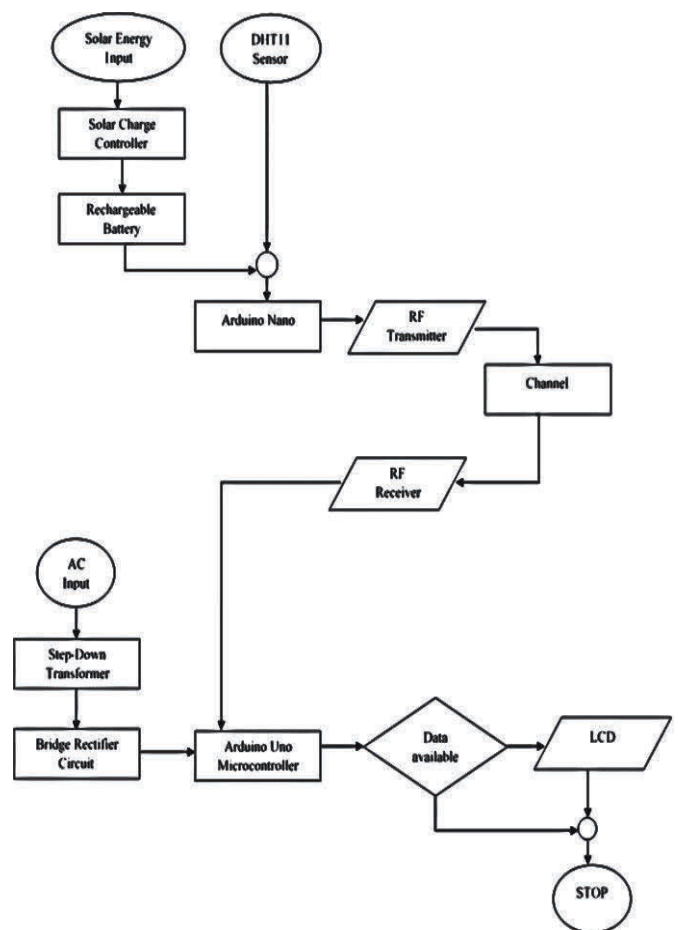
Fig 1: Renewable Power Source Weather Station Flow Chart
