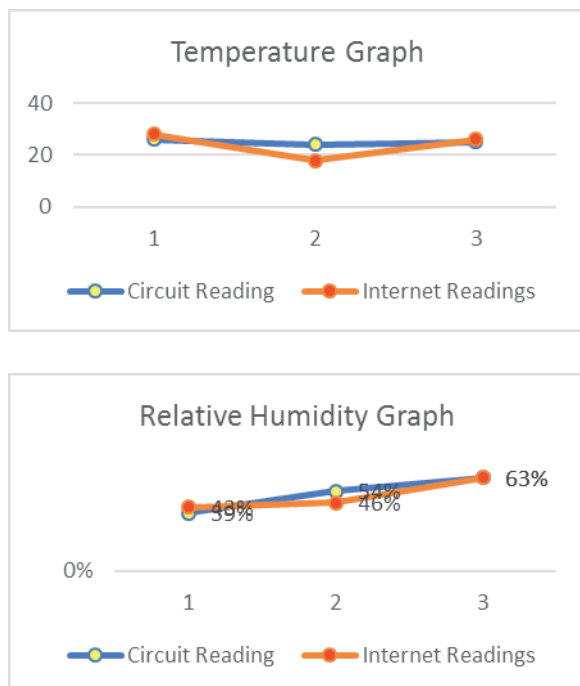
Fig 4: Graphs showing deviations of internet readings and the circuit readings
