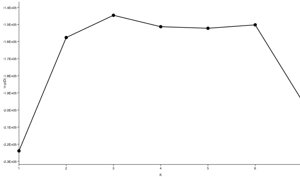
Fig. 2. Likelihood plot of STRUCTURE results. \ln P(D) is the mean likelihood of K , the number of simulated clusters. The most likely K is that where \ln P(D) is maximized.
