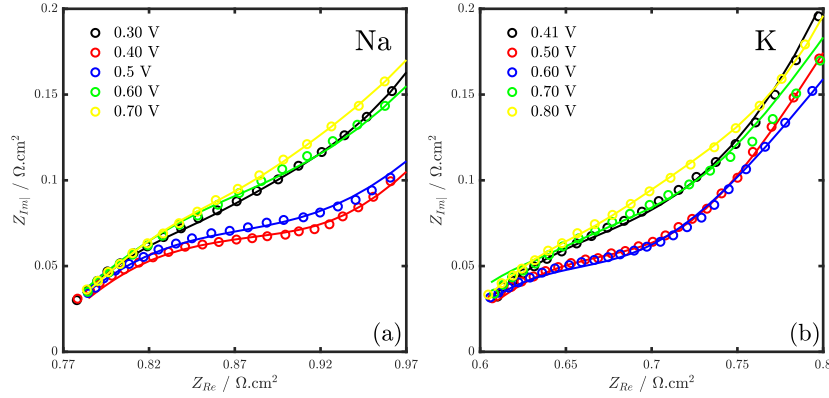
Figure 5: Nyquist plot of the high-frequency region of the impedance spectra obtained at different potentials during the anodic scan in 0.5 M (a) \text{Na}_2\text{SO}_4 and (b) \text{K}_2\text{SO}_4 .
