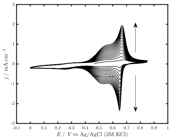
Figure 1: Cyclic voltammogram obtained during the electrodeposition of NiHCF in a freshly prepared solution of 2 mM \text{K}_3\text{Fe}(\text{CN})_6 , 2 mM \text{NiSO}_4 and 0.5 M \text{K}_2\text{SO}_4 using a scan rate of 25 \text{ mVs}^{-1} .
