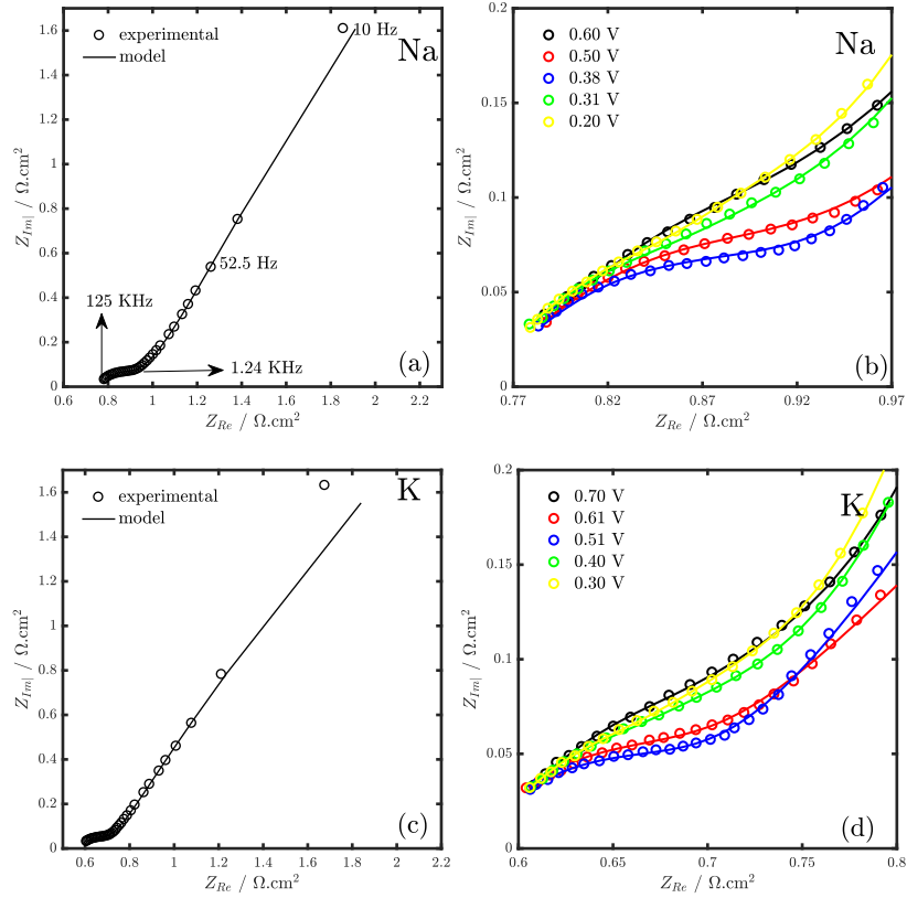
Figure 4: Nyquist plot of impedance spectra obtained in the cathodic scan of NiHCF thin film within the frequency range of 10 Hz to 125 KHz in (a) 0.5 M \text{Na}_2\text{SO}_4 solution at 0.38 V (b) High-frequency region of the impedance spectra obtained at different potentials during the cathodic scan in 0.5 M \text{Na}_2\text{SO}_4 (c) 0.5 M \text{K}_2\text{SO}_4 solution at 0.51 V (d) High-frequency region of the impedance spectra obtained at different potentials during the cathodic scan in 0.5 M \text{K}_2\text{SO}_4 .
