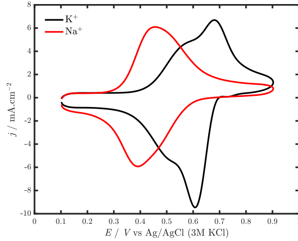
Figure 3: Cyclic voltammogram obtained from the quasi triangular wave applied to the NiHCF thin films in 0.5M A_2SO_4 solution ( A = K, Na ) using a scan rate of 200 \text{ mVs}^{-1} .
