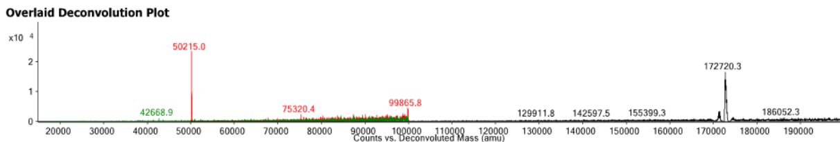
Figure 3 LC-MS spectra of the HTT N-HEAT_81-1643 domain.
