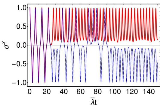
Figure 9. [Color online] Evolution of the order parameter \sigma^x(t) within the chaotic dynamical ferromagnetic phase C in Fig. 7, for g/\bar{\lambda} = 1.03 (solid red line) and 1.031 (dashed blue), and with J/\bar{\lambda} = 0.1 . Here N = 100 . The two lines are practically indistinguishable during the initial paramagnetic transient, but they have markedly distinct fates at the onset of the critical process denoted by (a) in the inset of Fig. 7 and they eventually end up into distinct wells. In both cases, \epsilon(t) grows from \epsilon(t=0) = 0 to values around 0.04 . This extreme sensitivity on the value of g (and of J ) is at the origin of the “mosaic” structure of region C in Fig. 7.
