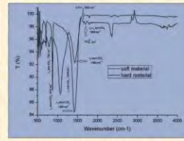
FTIR: Calcium sulphates as indicator of degradation
