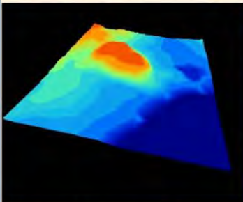
3D view of the DEM of the Barcelona surroundings (Z slightly exaggerated).
