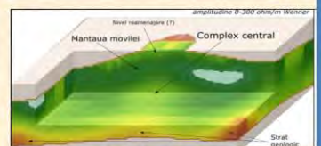
Three-dimensional model of electrical resistivity, Silvas
