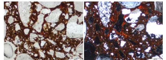
Progressive clogging of packing pores by micromass in Bt2 horizon of Nerets 1, resulting in a close porphyric c/f related distribution. Note also the clay coatings.
