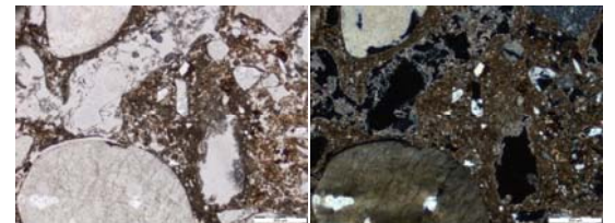
Loose discontinuous infilling of needle calcite in a channel (upper left) and micrite coating and impregnative hypocoating in a pore (lower right) in 2Bk horizon of Nerets 2.
