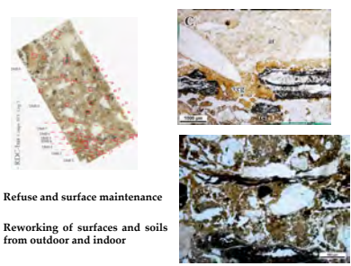
Dark earth, Metz (Borderie, Nicotia, Gebhardt 2016 C&CC-BY-NC)
