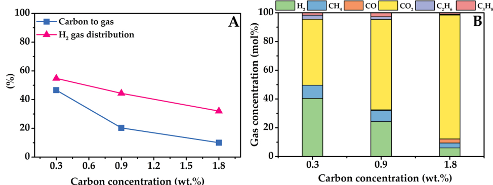
Fig. 5. Influence of the carbon concentration on APR performance of wheat straw hydrolysate (left) and composition of the produced gas phase (right). Reaction conditions: 0.375 g Pt/C catalyst, 2 h reaction time, 270 °C reaction temperature.
