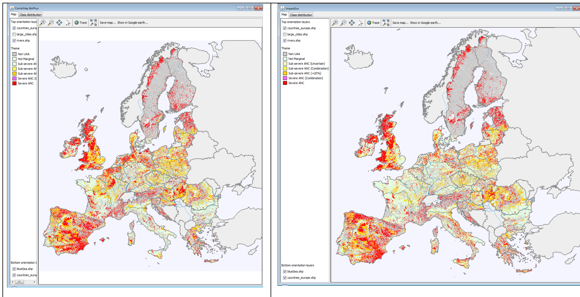
Map 1 Marginal lands based on biophysical constraints in EU-28 (marginal lands are in the 2 severe classes= Severe ANC and Severe ANC (combination)(red and purple)). Left map shows marginal lands without correction for improved lands/Right map show final map of marginal lands after correction for improved lands
