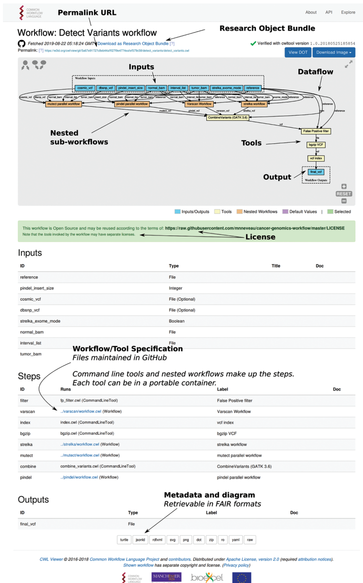
Figure 1. A workflow for detecting variants in genome sequences 5 . The workflow is specified in the Common Workflow Language, displayed using the CWL Viewer. Any CWL compliant WfMS execution engine should be able to execute this standardized workflow description and obtain the same results independent of their underlying infrastructure, for instance using Toil 6 executed on SLURM, or REANA 7 on Kubernetes.
