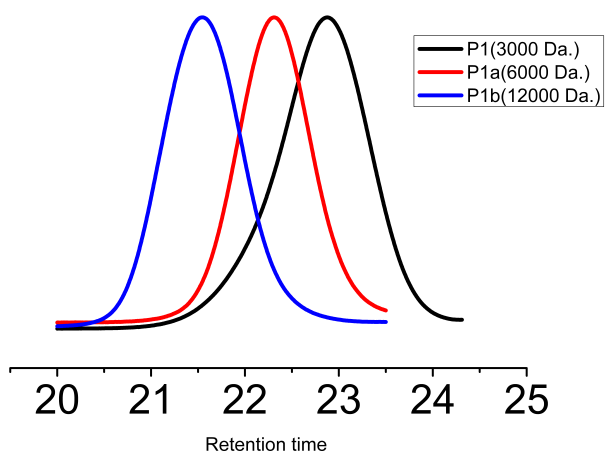
Figure 2. THF GPC elugram of the bifunctional initiated polymer using the M1 monomer.
