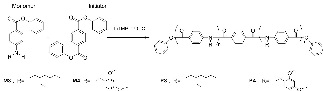
Figure 3. The chain growth polycondensation of M3 or M4 with a bifunctional initiator results in functionalizable telechelic polymers P3 and P4 .
