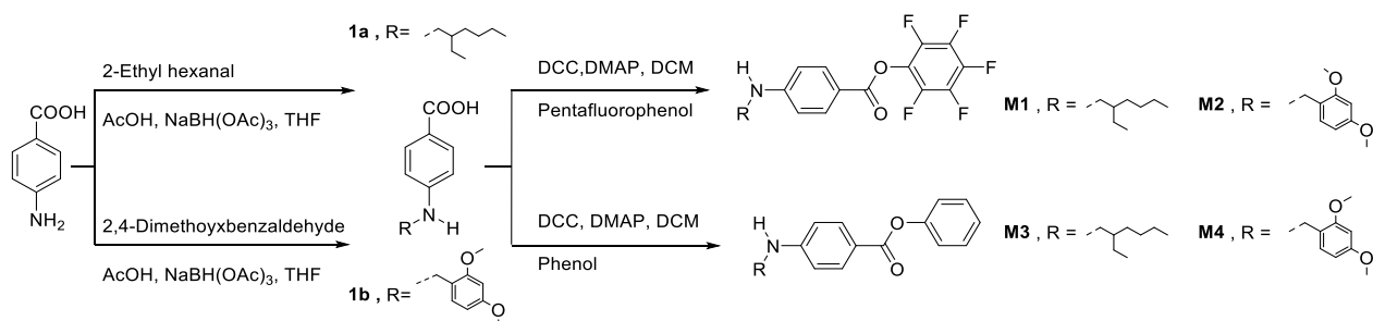
Figure 1. Synthesis of monomers M1-M4 .
