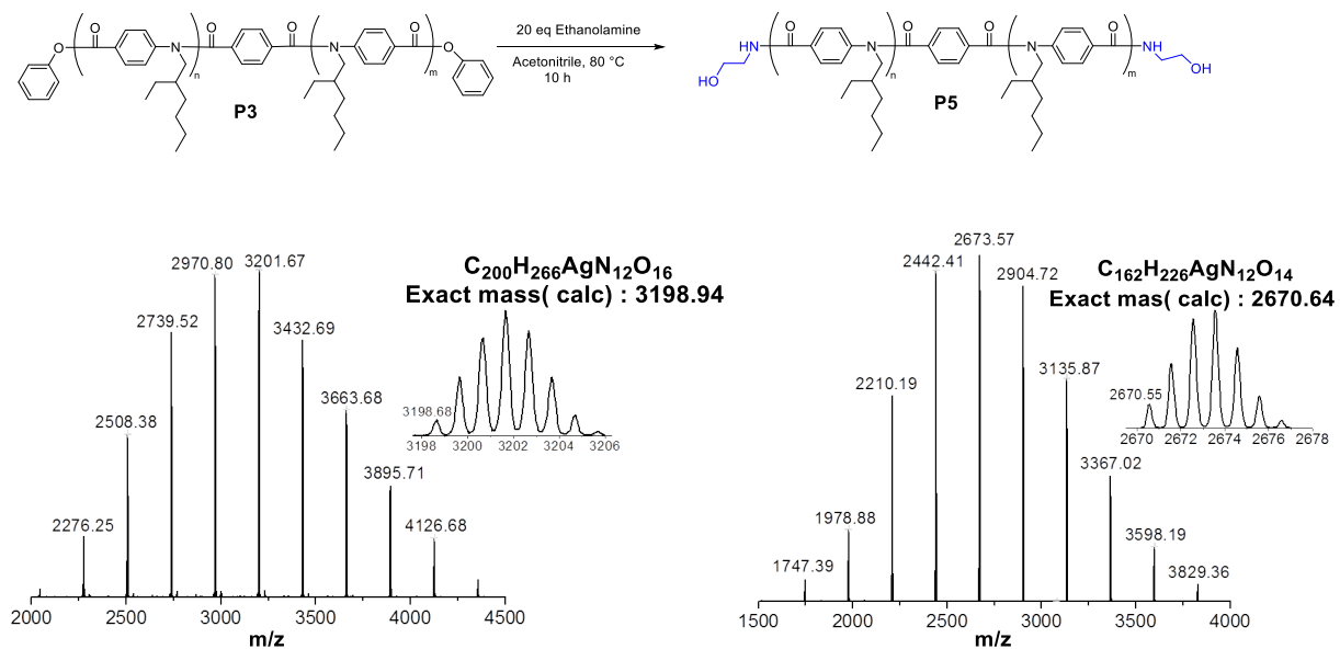
Figure 5. Left: MALDI-ToF mass spectrum of the bifunctional-initiated ethyl hexyl polymer P3 as an \text{Ag}^+ adduct. Right: MALDI-ToF mass spectrum of the modified bifunctional-initiated ethyl hexyl polymer P5 as an \text{Ag}^+ adduct. The insets show the most intense peak of the distribution isotopically resolved.
