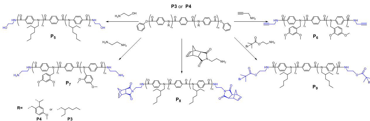
Figure 4. Post polymerization modification of P3 and P4 .
