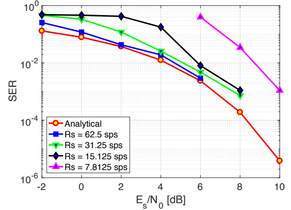
Fig. 11. Symbol Error Rate performance for the deep space scenario considering a 3rd order PLL + Costas, and a coherent subcarrier.
