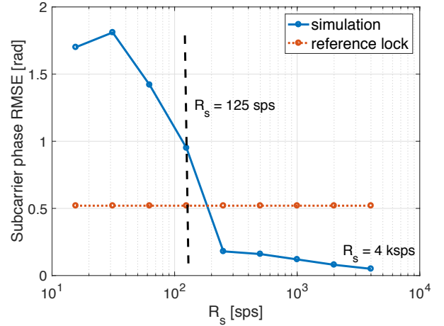
Fig. 4. Subcarrier phase RMSE versus symbol rate for the deep space scenario. Carrier Doppler rate = 1 Hz/s, subcarrier Doppler = 0.1 Hz, B_{pll} = 5 Hz, B_{Costas} = 5 Hz
