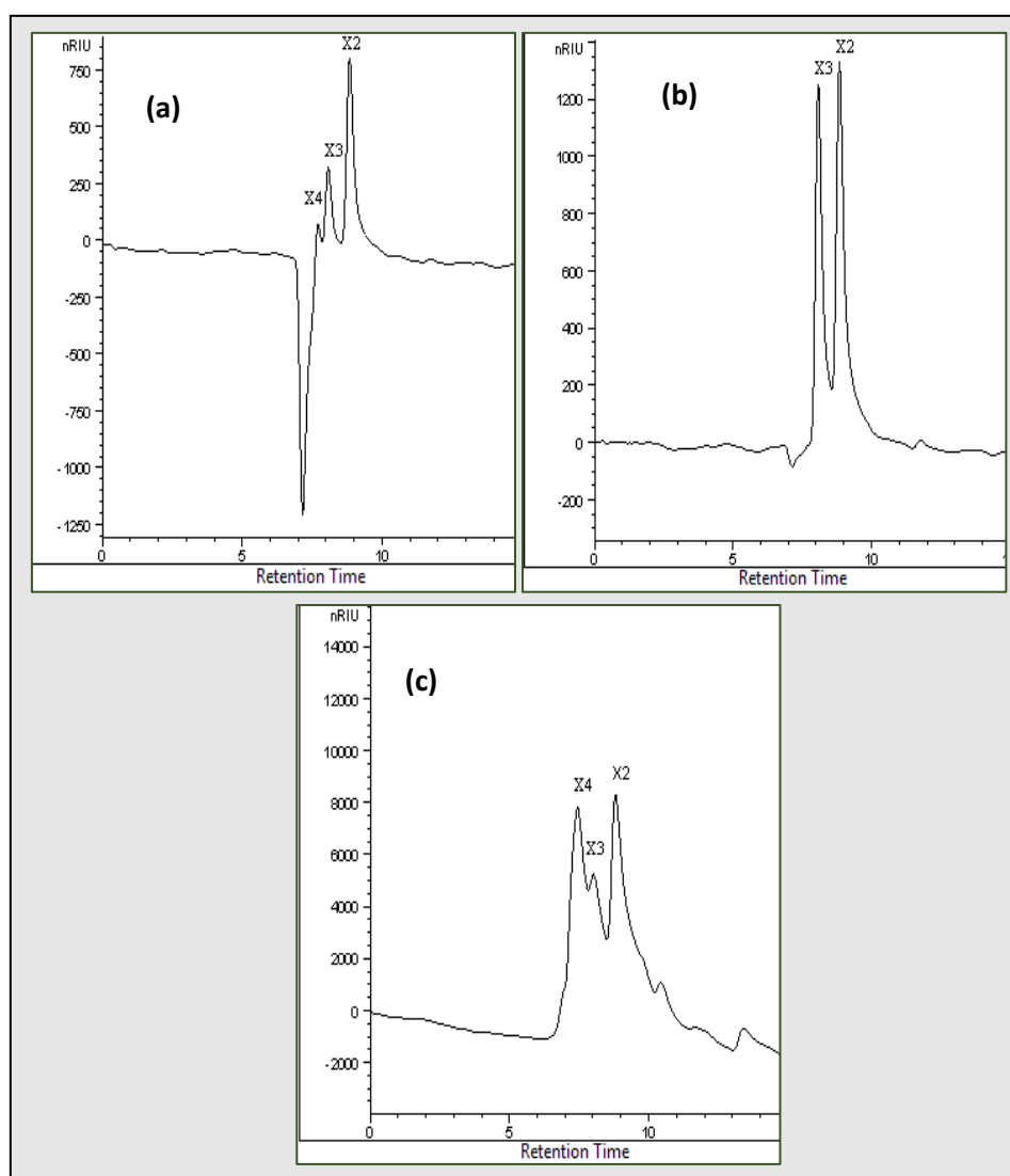
Figure S1. HPLC chromatograms of XOS produced from Saccharum officinarum L. by-products. X2: xylobiose; X3: xelotriose; X4: xylotetraose, (a) XOS standard; (b) XOS derived from Saccharum officinarum L. rind; (c) XOS derived from Saccharum officinarum L. pith
