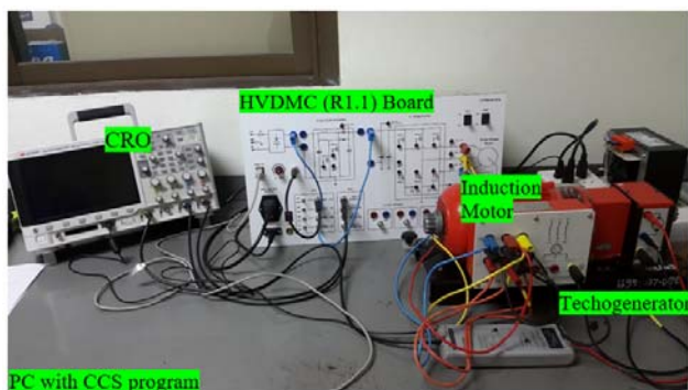
Fig. 7 Laboratory setup
