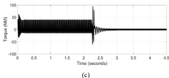
Fig. 8 (a) Speed, (b) current, (c) torque, and (d) voltage waveform for step change of speed setting
