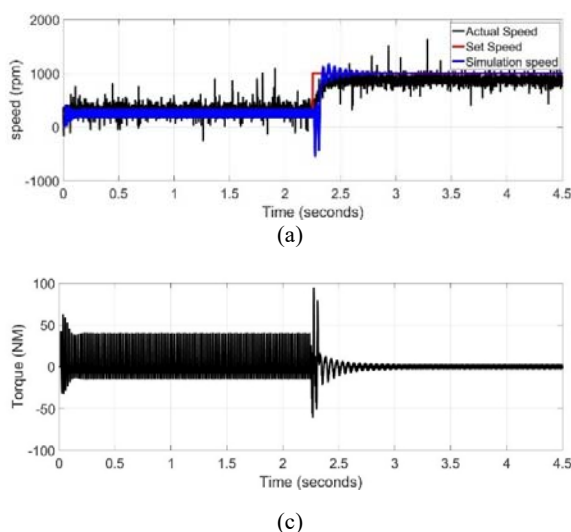
Fig. 8 (a) Speed, (b) current, (c) torque, and (d) voltage waveform for step change of speed setting
