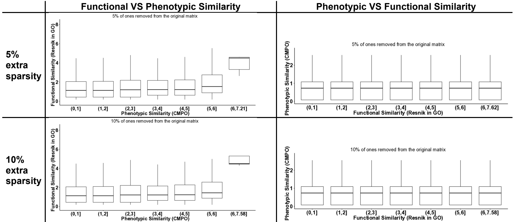
Figure S2. Distribution of functional similarity in GO versus phenotypic similarity (and vice versa) for different levels of sparsity.
