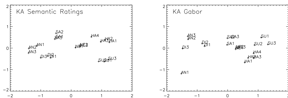
Figure 5. nMDS solutions for Gabor and semantic rating similarities (data from pilot study).
