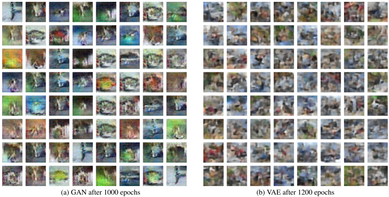
Figure 8: Generated images of a GAN and a VAE after training on CIFAR-10 dataset.
