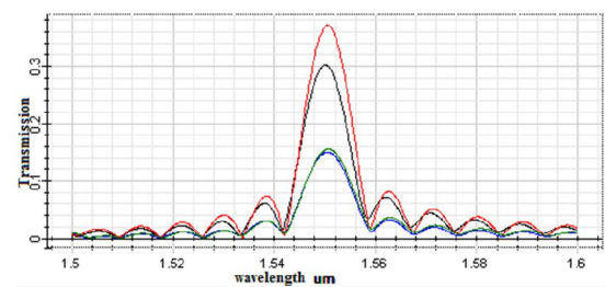
Fig 6: Output transmission of microcavity based biosensor.
