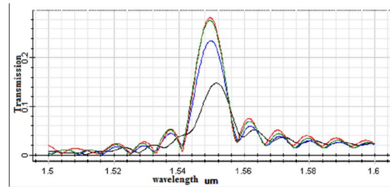
Fig 5: Output transmission spectrum of nanocavity based biosensor
