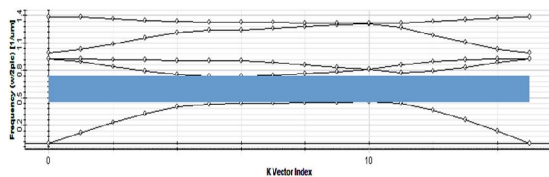
Fig 3: TE band diagram square lattice with defects
