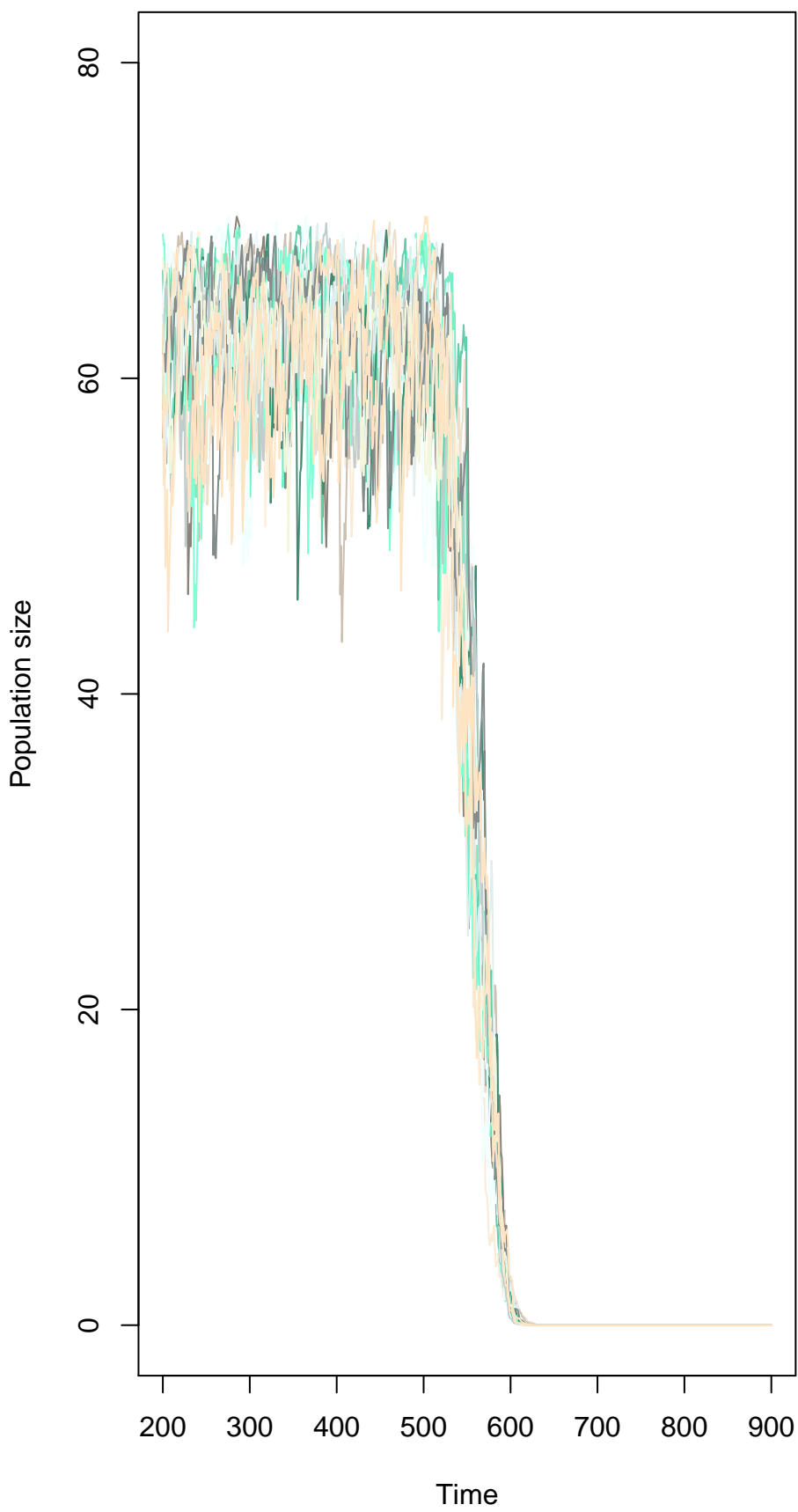
genetic variation = 0.05
