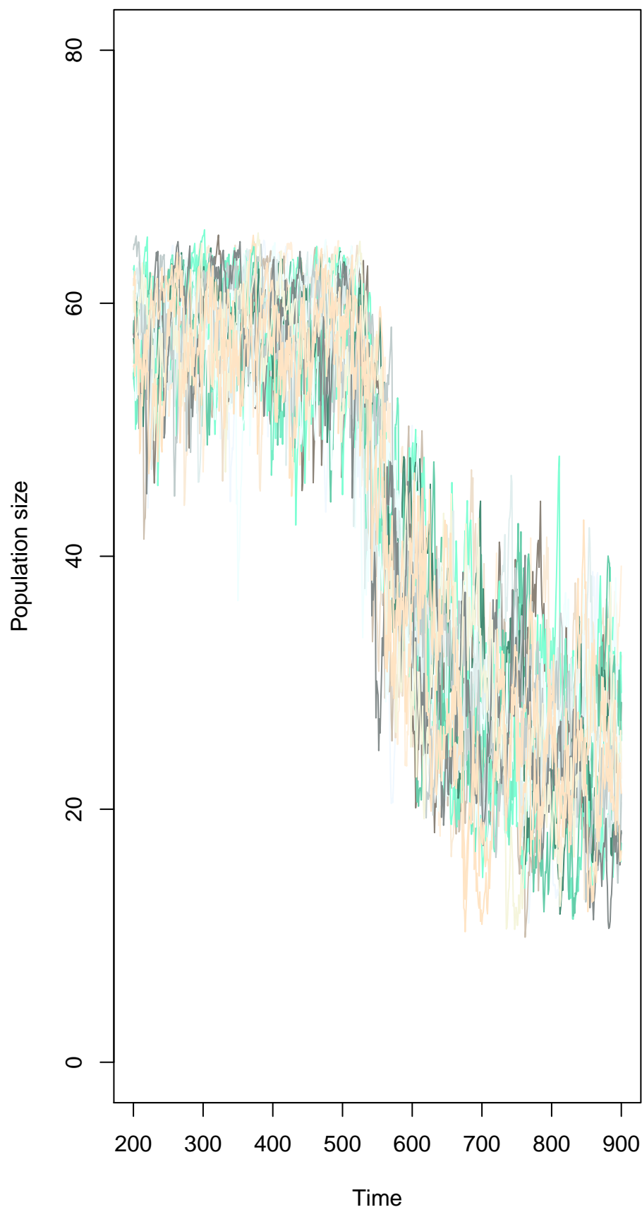
genetic variation = 0.5
