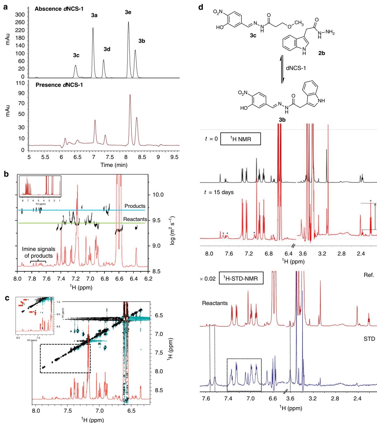
Fig. 4 HPLC-MS and NMR studies of the full dynamic combinatorial library. a DCL chromatograms after 5 h in the absence and in the presence of dNCS-1 . Conditions: aldehyde 1 (1.2 \mu\text{L} , 50 mM), 2a–2e (3.6 \mu\text{L} , 50 mM), catalyst (1 \mu\text{L} , 12 M), dNCS-1 : 1 [1:1], Tris buffer (20 mM, pH 7.4), 1 mM \text{CaCl}_2 , 0.5 M NaCl, 1 mM DTT, T = 4^\circ\text{C} , 2% DMSO. DCC experiments were carried out in triplicate. b 1D- ^1\text{H} NMR spectrum (red) of the mixture and DOSY experiment (black) of the DCL in the presence of dNCS-1 (281 K, 600 MHz). c Tr-NOESY spectrum of the DCL mixture in the presence of dNCS-1 (mixing time 200 ms, 281 K, 600 MHz). Amplification of the region \delta 7.2–8.0 ppm. The negative transferred NOE cross-peaks corresponding to intramolecular NOEs of the products while bound to the protein are highlighted with red solid arrows. d ^1\text{H} -NMR spectrum of the sample with acylhydrazide 2b and acylhydrazone 3c in the presence of dNCS-1 at different reaction times and up to 15 days (281 K, 600 MHz). The new signals that reveal the formation of 3b (aromatic region) and 2c (aliphatic region) are marked with stars. ^1\text{H} -STD-NMR (blue) and off-resonance (red) NMR spectra of the mixture 2b + 3c + dNCS-1 (281 K, 600 MHz) after 15 days
