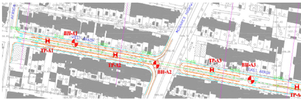
Fig. 7 The plan of bore holes and test pit location
