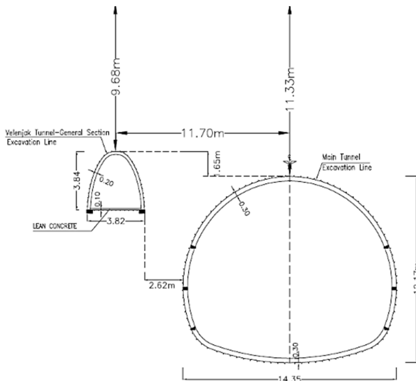
Fig. 3 The geometrical properties of the numerical model (The Africa tunnel next to Velenjak sewer)
