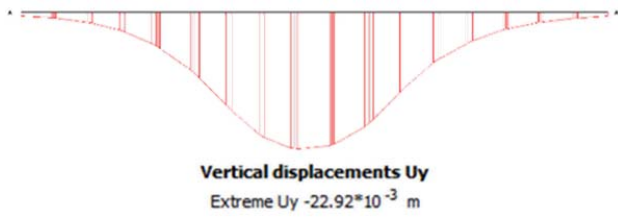
Fig. 16 The induced vertical displacement at the ground surface (based on the revised properties)
