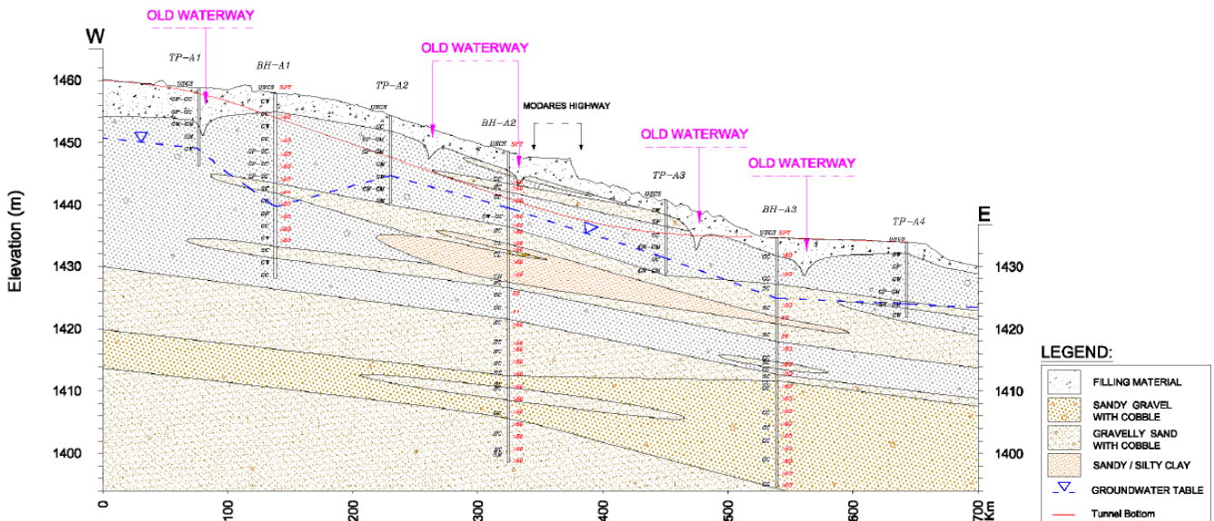
Fig. 8 Schematic geological layers of the project site
