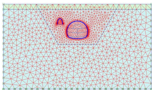
Fig. 5 The generated finite element mesh used for the analysis
