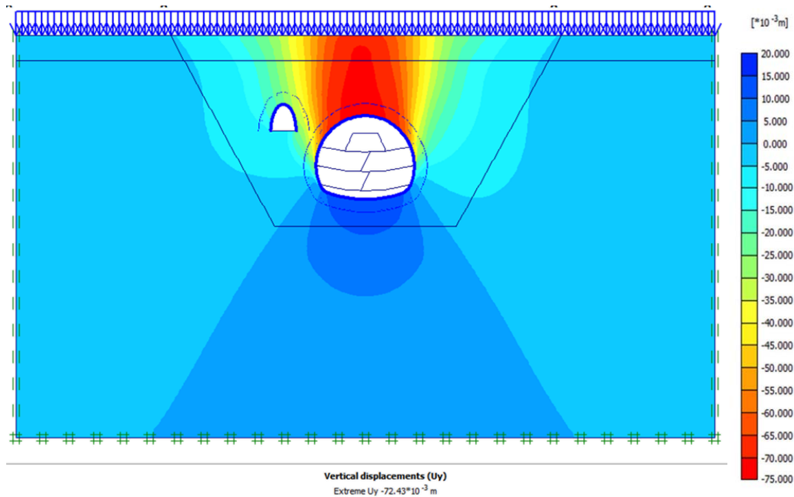
Fig. 11 The induced vertical displacement at the end of construction (based on primitive properties)
