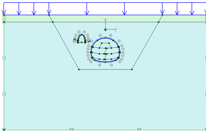
Fig. 4 The developed numerical model
