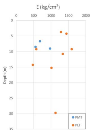
Fig. 14 The variations of modulus of elastic deformation vs. depth of soil sample based on PMT and PLT
