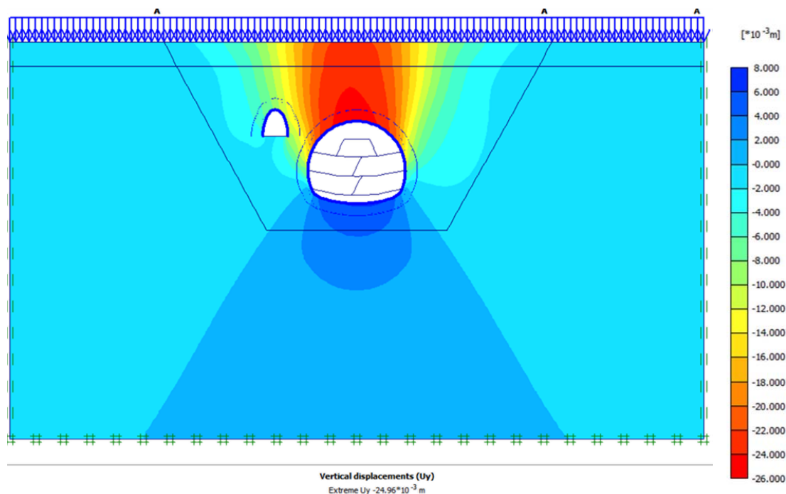
Fig. 15 The induced vertical displacement at the end of construction (based on the revised properties)
