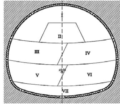
Fig. 6 The sequence of the tunnel excavation (The Africa tunnel)
