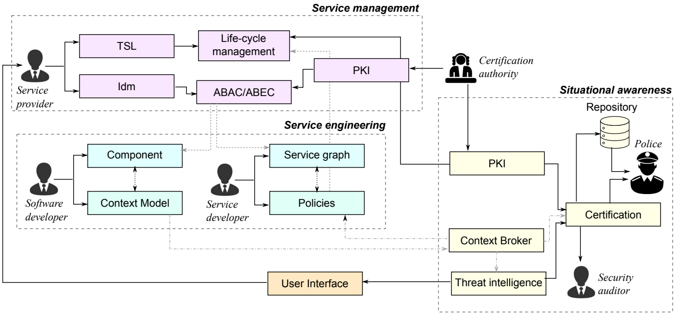
Fig. 3: The ASTRID framework.
