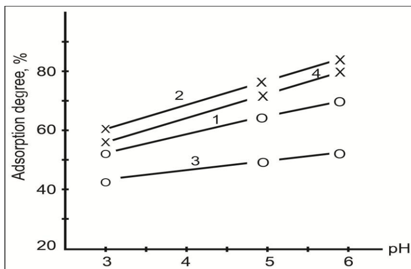
Fig 2:- Impact of environment pH on adsorption degree of \text{Cu}^{2+} and \text{Fe}^{2+}
