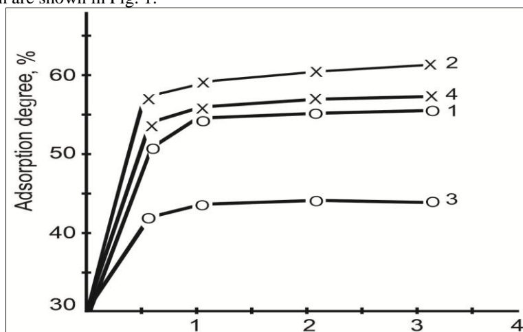
Fig 1:- Contact time influence on adsorption degree for \text{Cu}^{2+} and \text{Fe}^{2+}
